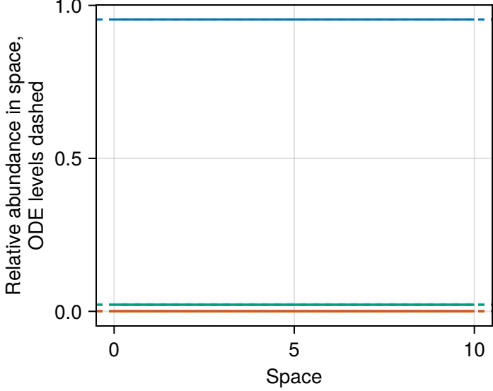
Community composition across space
