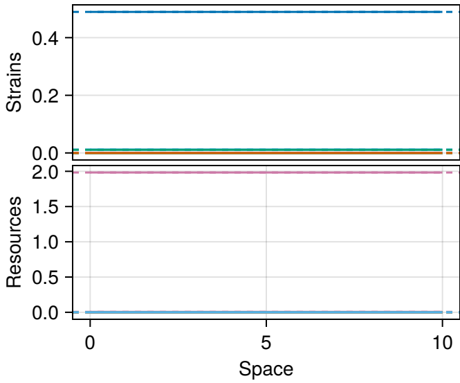
PDE final states
