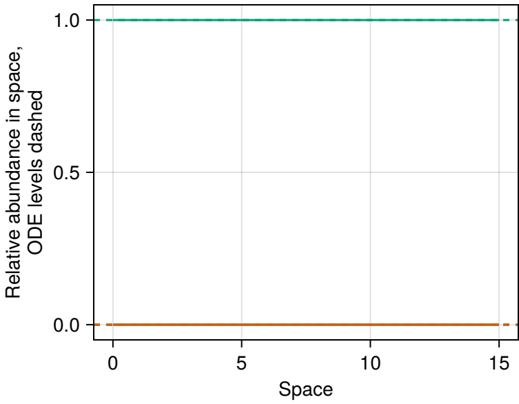
Community composition across space
