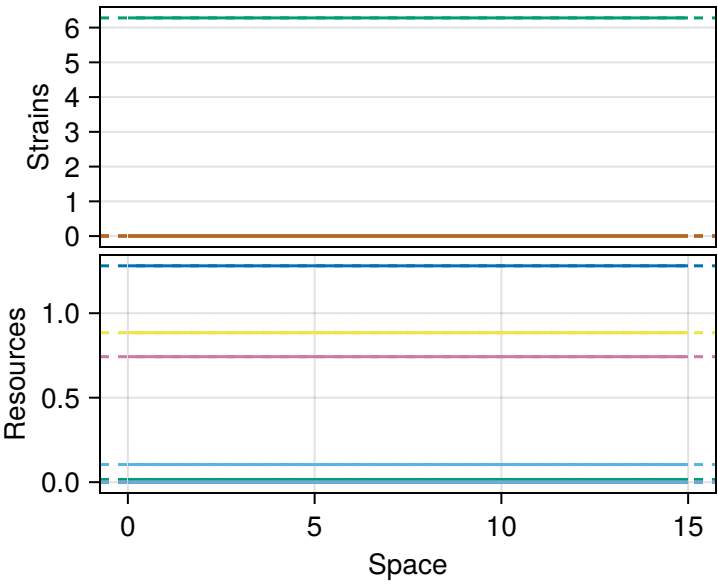
PDE final states
