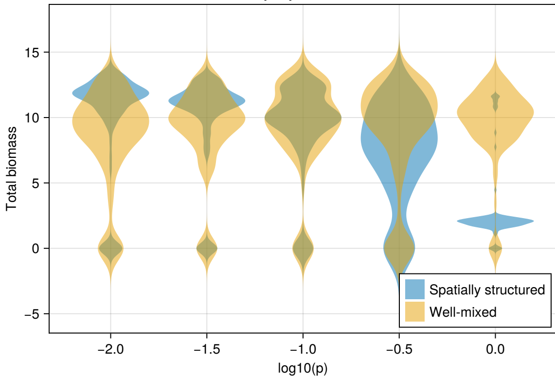
Total biomass distributions for different p (ODEs and PDEs), 100 runs per p , K=15.0 , I=0.999
