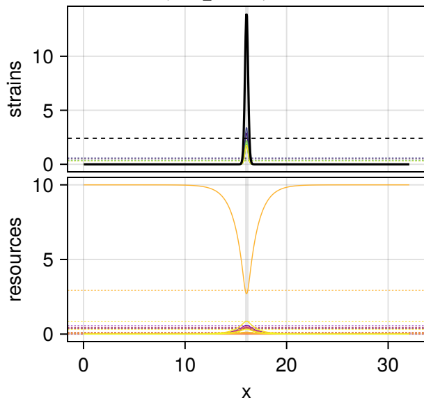
relamp 81.03, FWHM 0.01 L Success, final_T 1e+08 , maxresid 2.6e-12
