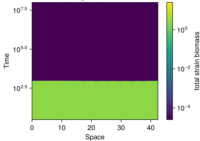
row 24, sys 12, p = 10 L = 42.4 , N_s = 6 Success, final_T 1e+08 , maxresid 2.3e-23
