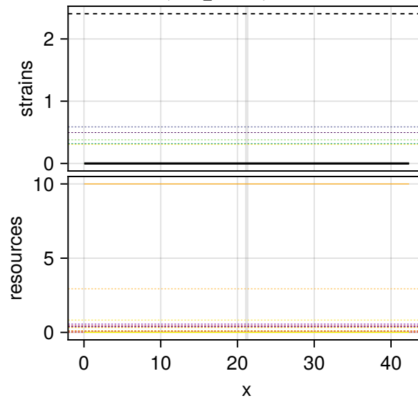
relamp 12.37, FWHM 0.01 L Success, final_T 1e+08 , maxresid 2.3e-23
