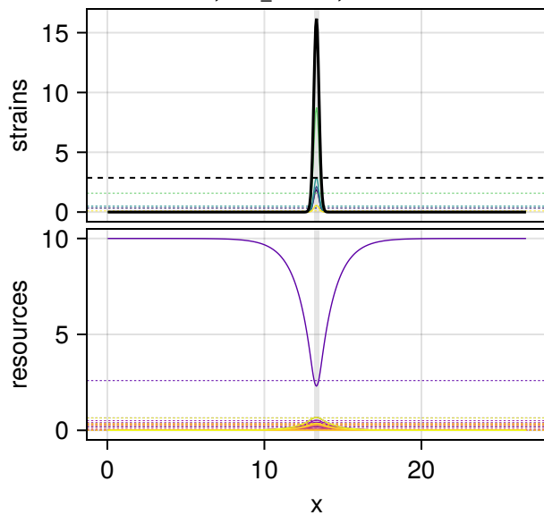
relamp 64.46, FWHM 0.01 L Success, final_T 1e+08 , maxresid 2.0e-12
