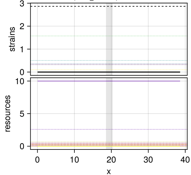
relamp 18.64, FWHM 0.05 L Success, final_T 1e+08 , maxresid 2.4e-31
