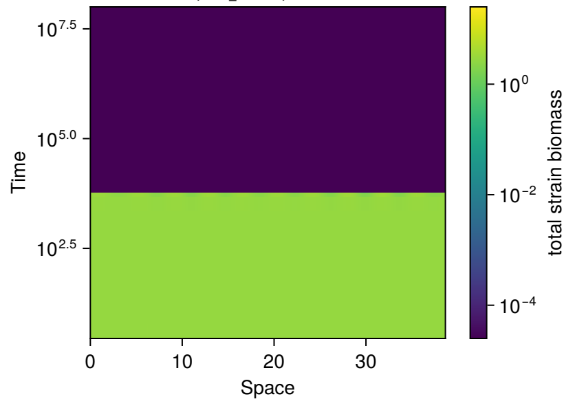
row 30, sys 15, p = 10 L = 38.6 , N_s = 5 Success, final_T 1e+08 , maxresid 2.4e-31
