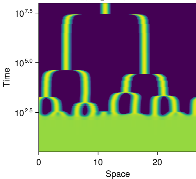
row 29, sys 15, p = 1 L = 26.7 , N_s = 5 Success, final_T 1e+08 , maxresid 2.0e-12
