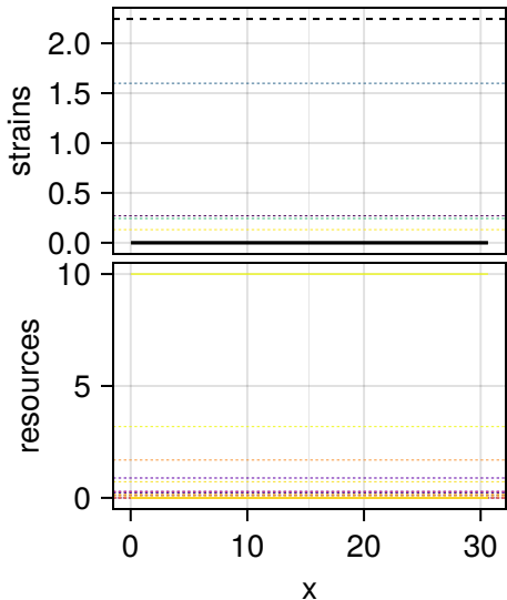
row 16, sys 8, p = 10 relamp 11.52, FWHM 0.00 L Success, final_T 1e+08, maxresid 4.4e-26
