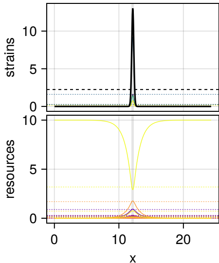
row 15, sys 8, p = 1 relamp 60.30, FWHM 0.02 L Success, final_T 1e+08, maxresid 1.3e-12
