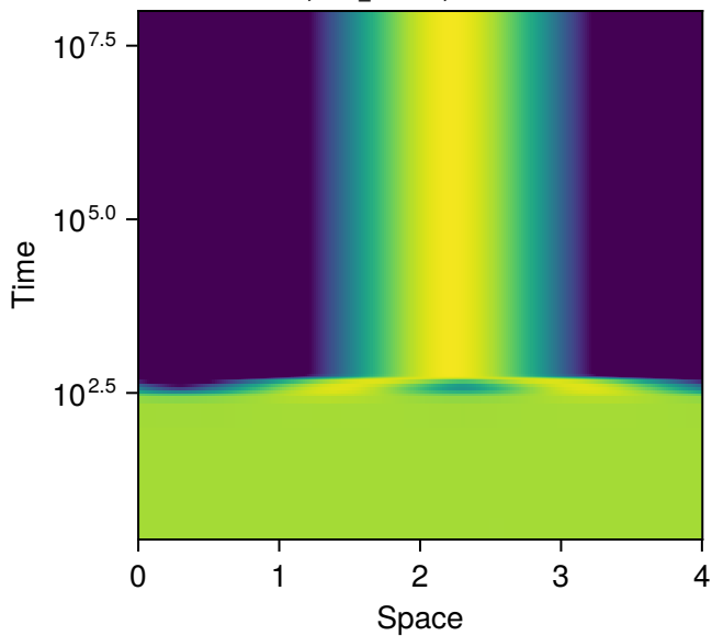
row 3, sys 2, p = 1 L = 4 , N_s = 3 Success, final_T 1e+08 , maxresid 8.7e-11
