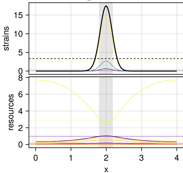
relamp 9.25, FWHM 0.10 L Success, final_T 1e+08 , maxresid 8.7e-11
