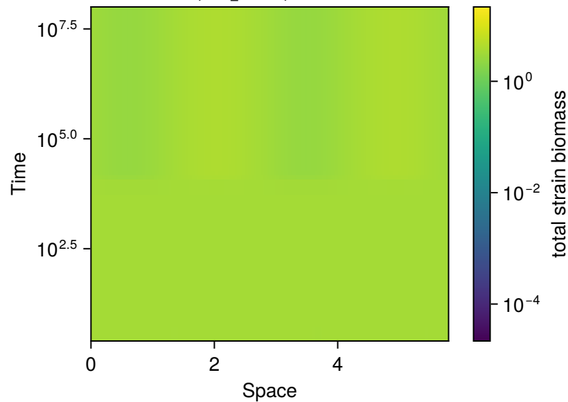
row 4, sys 2, p = 10 L = 5.8 , N_s = 3 Success, final_T 1e+08 , maxresid 4.0e-12
