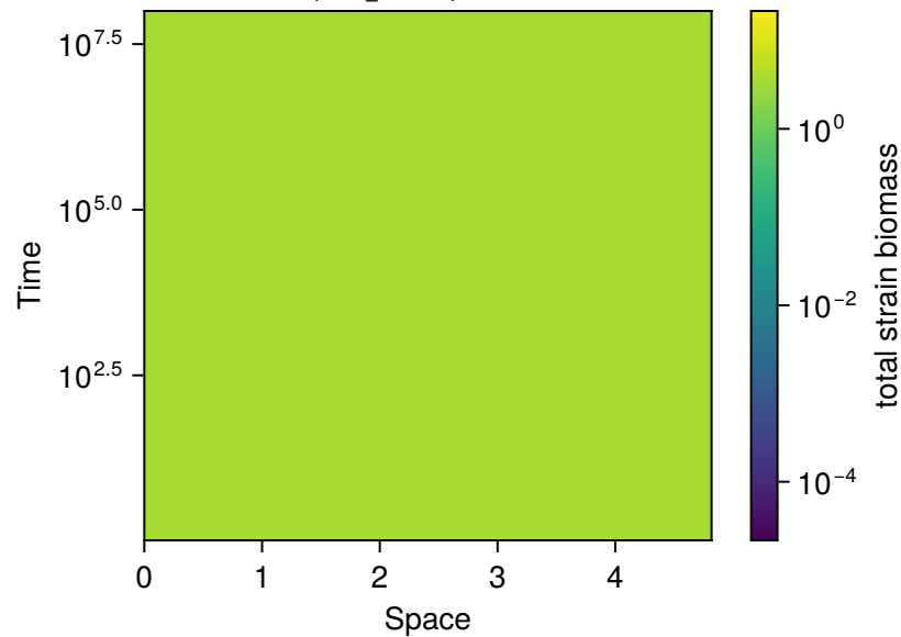
row 24, sys 12, p = 10 L = 4.82 , N_s = 7 Success, final_T 1e+08, maxresid 3.0e-12
