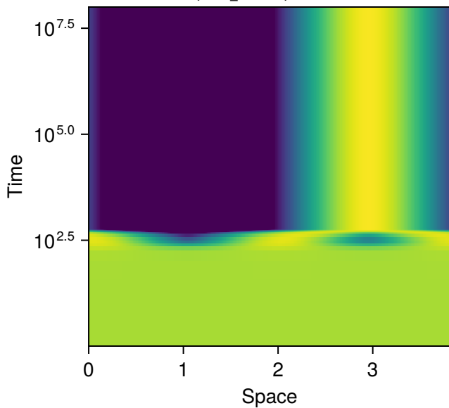
row 23, sys 12, p = 1 L = 3.82 , N_s = 7 Success, final_T 1e+08, maxresid 6.5e-12
