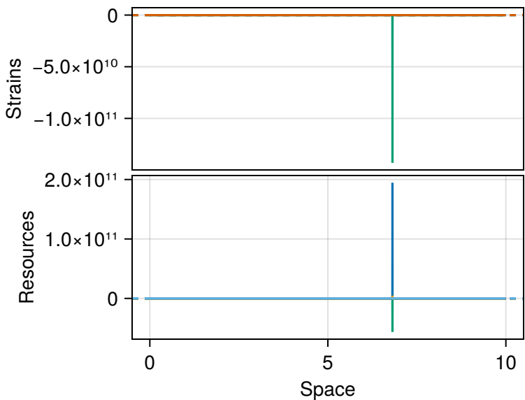
PDE mean abundances
