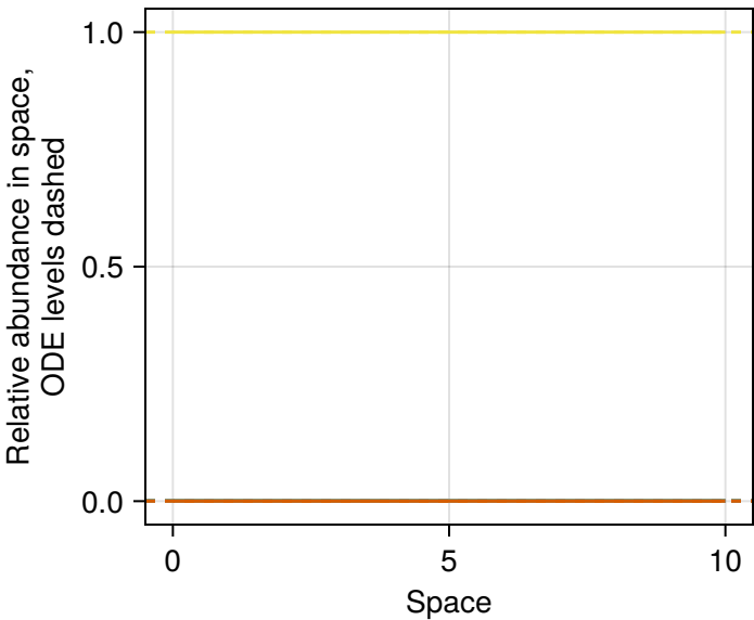
Relative abundance in space, ODE levels dashed
