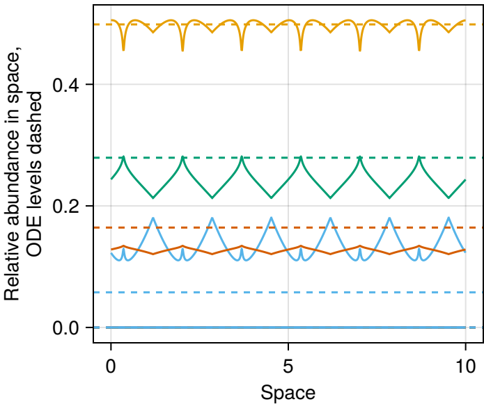
Community composition across space
