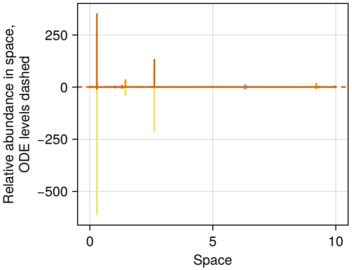
Community composition across space
