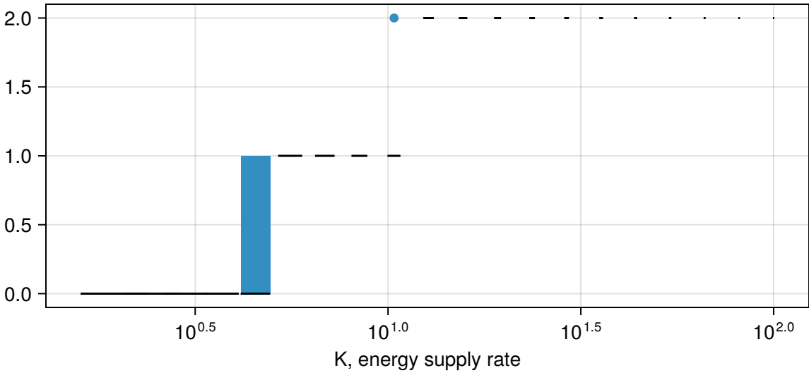
cooperativity k=0.1
