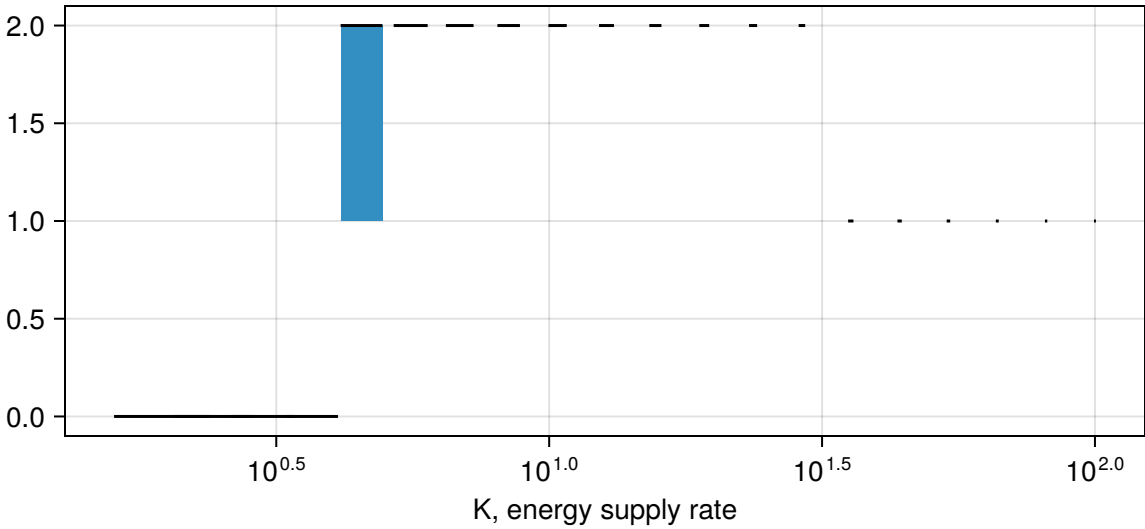
cooperativity k=0.001
