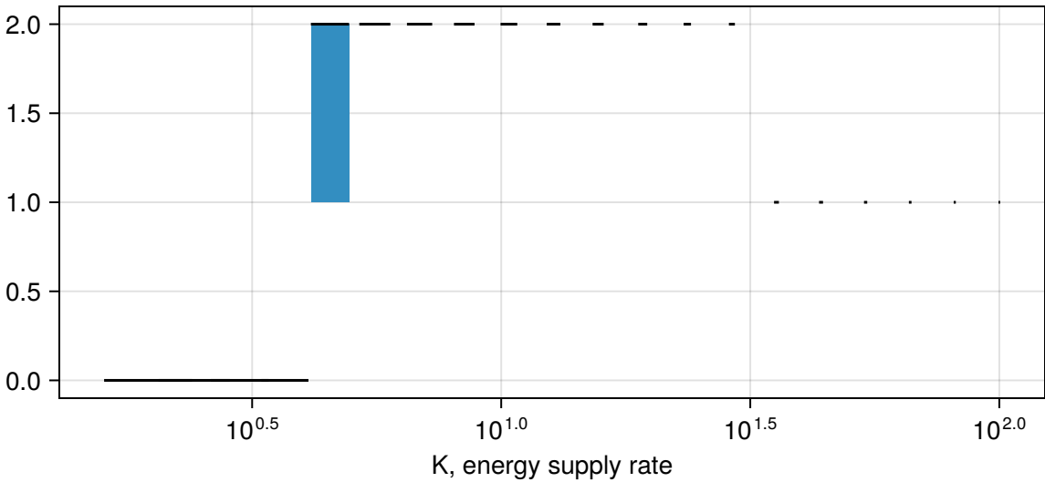
cooperativity k=0
