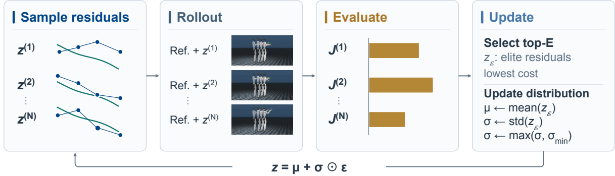
Figure 3 Sampling-based command optimization (SCO) uses CEM to optimize sparse pose residuals through sampling, rollout, evaluation, and proposal updates. (a) Receding-horizon correction with a planning horizon and executed prefix. (b) The CEM loop proceeds from sampling to rollout, evaluation, and distribution update; the feedback arrow returns to sampling.
