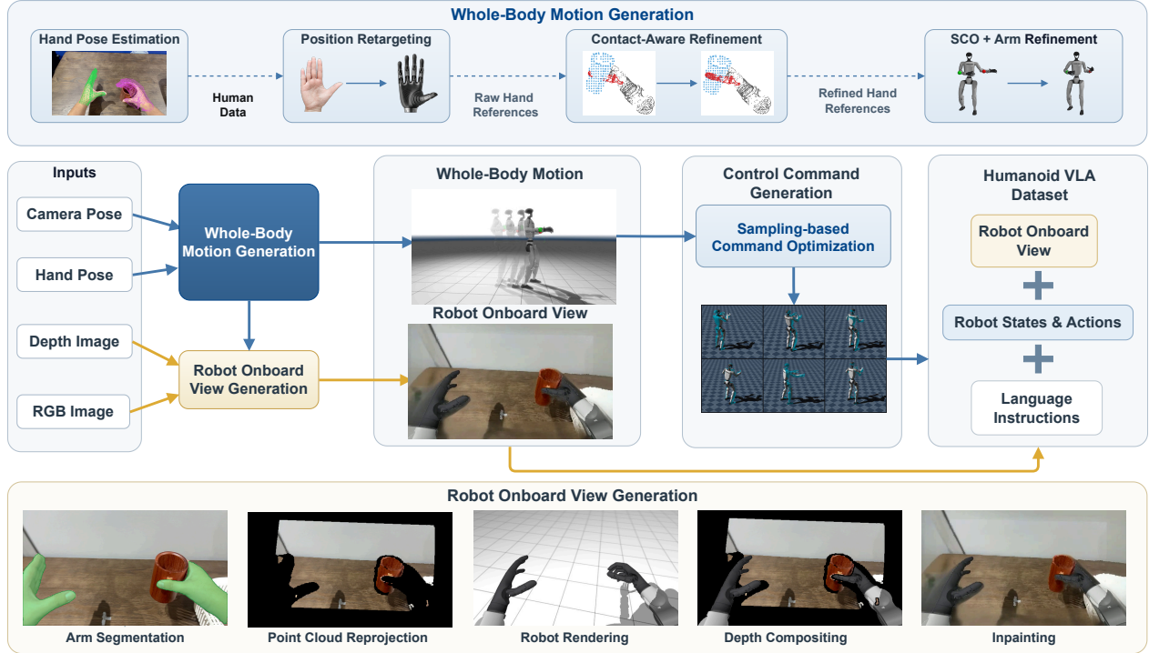
Figure 2 KODA pipeline. Middle: Human demonstrations become aligned whole-body motion and onboard observations, then controller-specific state-action data for VLA training (Control Command Generation). Top: Whole-Body Motion Generation combines hand estimation and contact-aware retargeting, sampling-based command optimization (SCO), and arm refinement. Bottom: Robot Onboard View Generation combines arm removal, scene reprojection, robot rendering, depth compositing, and inpainting. Input depth is observed or estimated from RGB.
