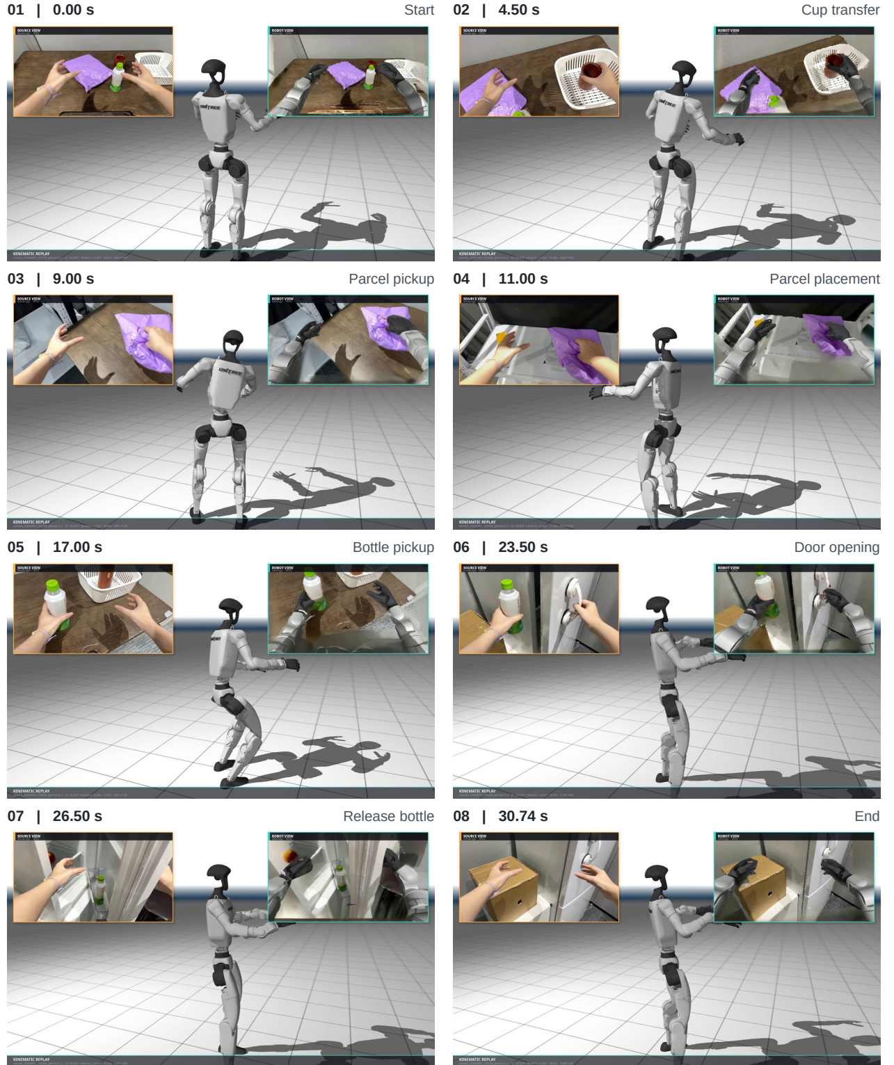
Figure E.2 Complete-clip timeline: sequential object manipulation. Eight selected moments span a 30.76 s clip: a cup is moved toward a basket, a parcel is transferred to a shelf, and a bottle is carried to a refrigerator and placed inside before the door is closed. The first and last video frames are included. Time advances left to right and then top to bottom; the three synchronized displays have the same meanings as in Fig. E.1.
