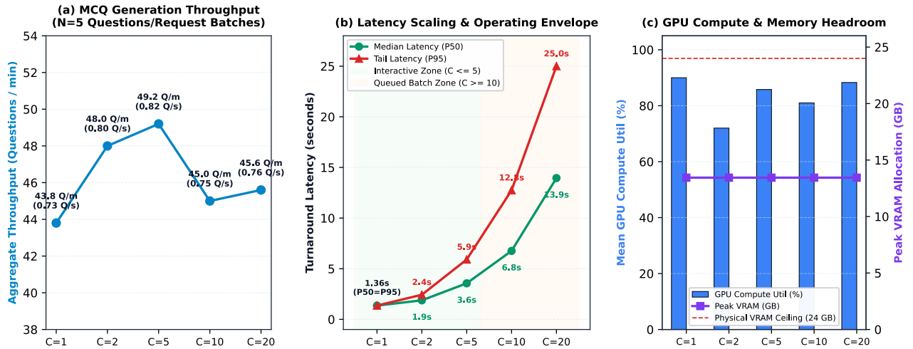
Figure 6: Single-GPU concurrency operating envelope and resource headroom on a dedicated NVIDIA RTX 3090 host (Experiment 4). (a) Aggregate throughput in questions/min across concurrency tiers C = 1 \dots 20 under standardized 5-question request batches, showing saturation at 43.8–49.2 Q/min. (b) Median (P50) and tail (P95) latency scaling, highlighting the interactive faculty authoring envelope ( C \leq 5 , latency \leq 3.56 s) versus queued batch saturation ( C \geq 10 ). (c) Host resource allocation showing mean GPU compute utilization and peak VRAM safely contained at 13.44 GB against the 24 GB hardware ceiling.
