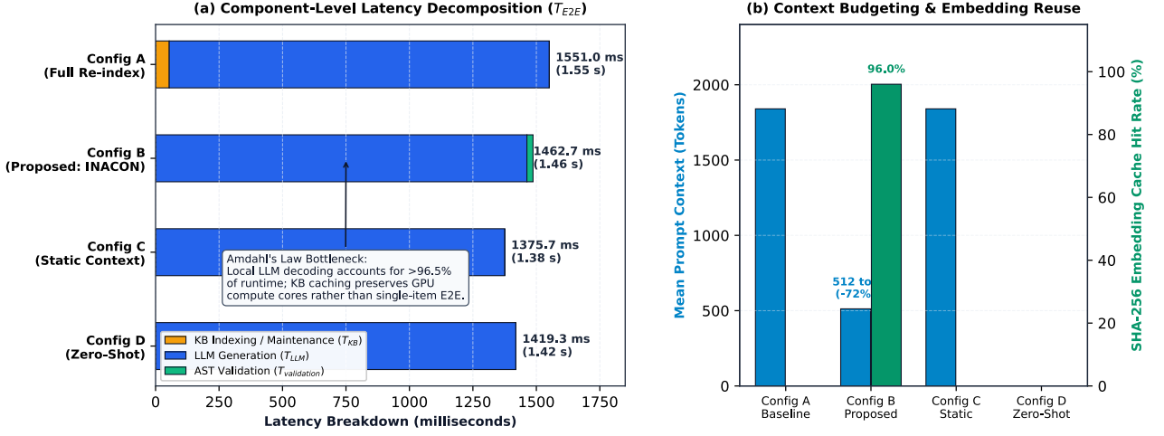
Figure 4: Pipeline component ablation and latency breakdown (Experiment 2). (a) Component-level latency decomposition ( T_{E2E} ) across baseline (Config A), proposed INACON pipeline (Config B), static context (Config C), and zero-shot generation (Config D), illustrating Amdahl's Law constraint where local LLM autoregressive decoding dominates >96.5% of execution time. (b) Trade-off between prompt context tokens and SHA-256 chunk embedding cache-hit rates, highlighting the 72.2% context compression achieved by bounded semantic retrieval.
