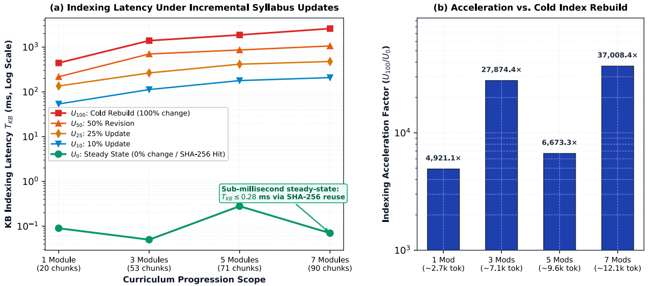
Figure 5: Knowledge Base indexing latency and scalability across curriculum progression scales and update ratios (Experiment 3). (a) Indexing latency T_{KB} (log scale) from 1 to 7 modules under update conditions U_0 through U_{100} , showing sub-millisecond steady-state performance ( T_{KB} \leq 0.28 ms). (b) Empirical speedup factor of SHA-256 incremental embedding reuse over cold rebuilds ( U_{100}/U_0 ), scaling from 4,921.1× to 37,008.4×.
