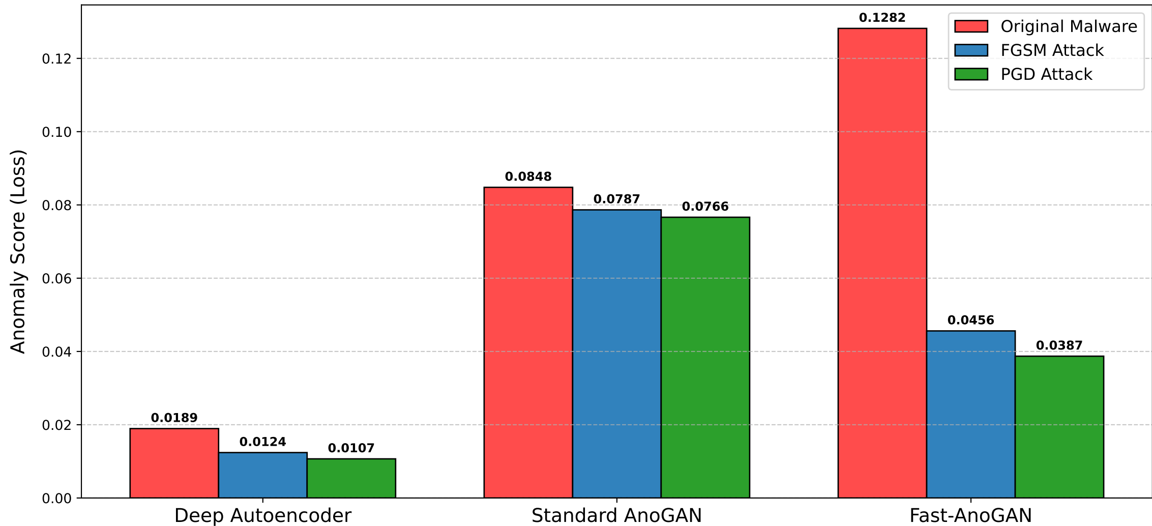
Attack Comparison (UNSW): Baseline vs FGSM vs PGD
