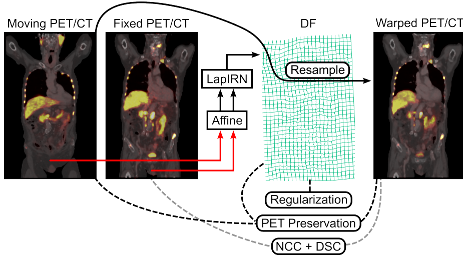
Fig. 1. Overview of the proposed registration pipeline. The moving (follow-up) and fixed (baseline) PET/CT are first coarsely aligned by an affine pre-registration (red), and the affinely aligned pair is passed to the coarse-to-fine LapIRN network, which predicts a dense displacement field (DF, green grid) used to resample the moving scan into the fixed space (warped PET/CT). Training is driven by three groups of objectives: deformation regularisation on the DF, comprising a global smoothness and folding penalty and a per-structure bone-rigidity term that constrains the DF inside skeletal labels and thereby also acts as an anatomical surrogate for biomarker preservation, since a large fraction of the lesion volume is intraosseous; PET-biomarker preservation terms (MTV, TLG and Jacobian inside the tumour mask) comparing the moving and warped lesions (black dashed); and image- and label-based similarity, NCC and DSC, between the fixed and warped scans (grey dashed). At test time, the same objectives are descended per pair by instance optimisation (IO).
