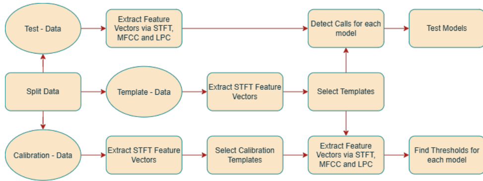
Figure 4.1: Zoomed out image of System Design
