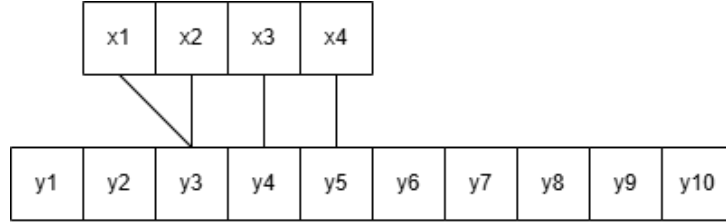
Figure 2.3: Example of a subsequence DTW alignment between two signal X = [x_1, x_2, x_3, x_4] and Y = [y_1, y_2, y_3, y_4, y_5, y_6, y_7, y_8, y_9, y_{10}]
