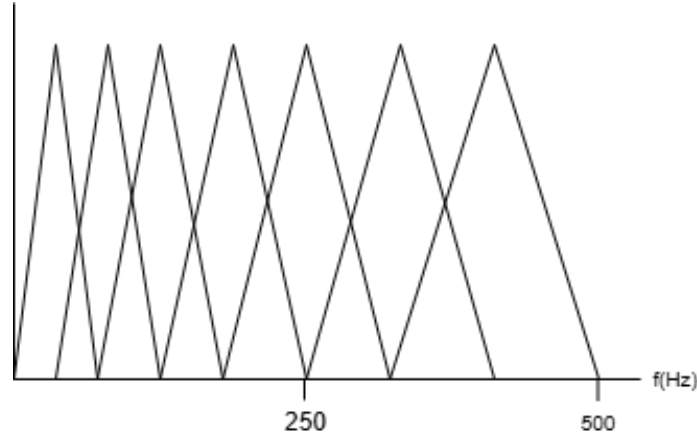
Figure 2.4: The mel scale filter bank is made up of 20 to 40 triangular filters arranged according to the mel scale.
