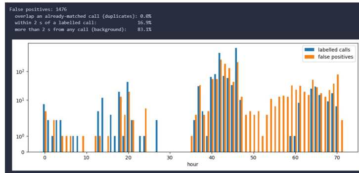
Figure 6.7: Timeline of audio file 22 showing where the most False Positives occur in relation to the actual calls
