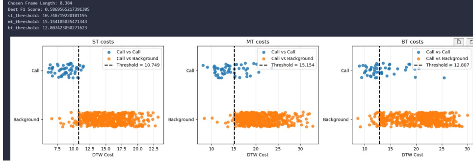
Figure 6.9: Scatter plot showing threshold placement in terms of background images and call templates
