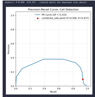
Figure 6.10: Precision vs Recall curve
