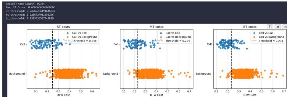
Figure 6.1: Scatter plot showing threshold placement in terms of background images and call templates
