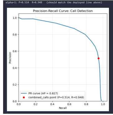
Figure 6.6: Precision vs Recall curve
