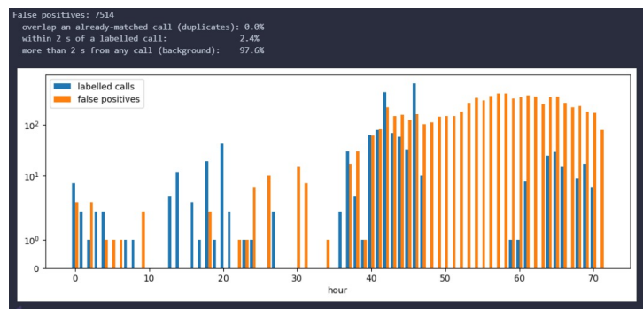
Figure 6.15: Timeline of audio file 22 showing where the most False Positives occur in relation to the actual calls
