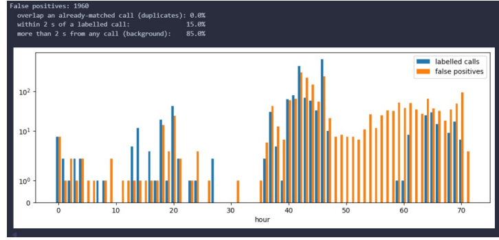
Figure 6.3: Timeline of audio file 22 showing where the most False Positives occur in relation to the actual calls
