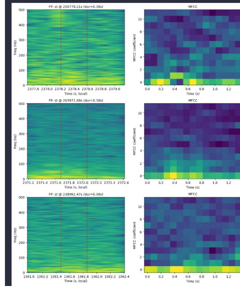
Figure 6.12: Spectrograms of False Positive calls. Many of which could actually be real calls
