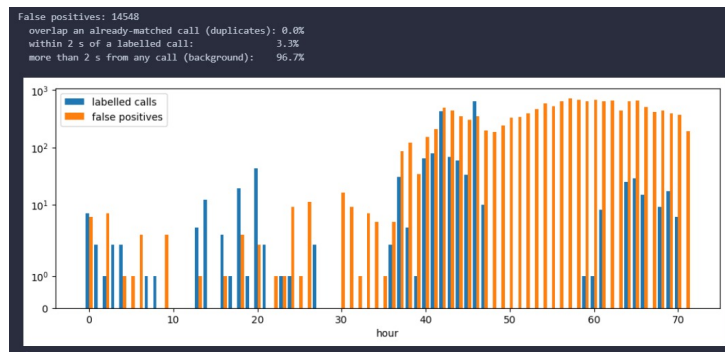
Figure 6.11: Timeline of audio file 22 showing where the most False Positives occur in relation to the actual calls
