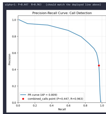
Figure 6.2: Precision vs Recall curve
