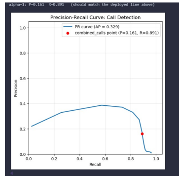
Figure 6.14: Precision vs Recall curve
