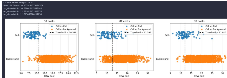
Figure 6.13: Scatter plot showing threshold placement in terms of background images and call templates
