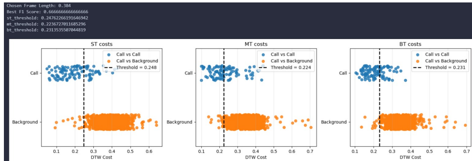
Figure 6.5: Scatter plot showing threshold placement in terms of background images and call templates
