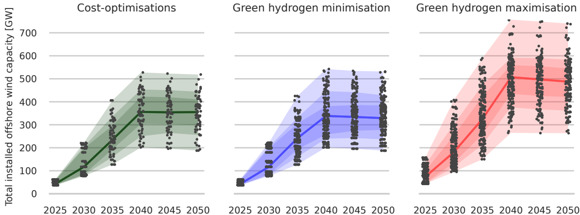
(c) Total installed offshore wind capacity
