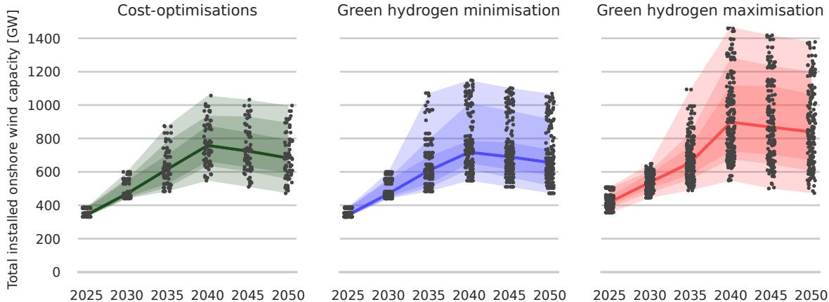
(b) Total installed onshore wind capacity
