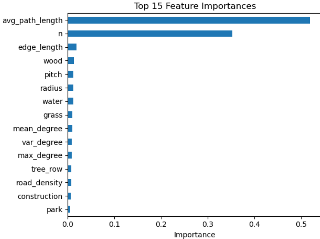
Figure 7: The 15 most important features in the reduced model.
