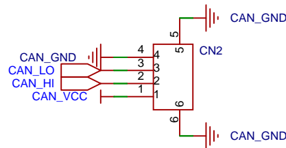
BM04B-GHS-TBT(LF)(SN)
