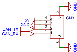
BM04B-GHS-TBT(LF)(SN)
