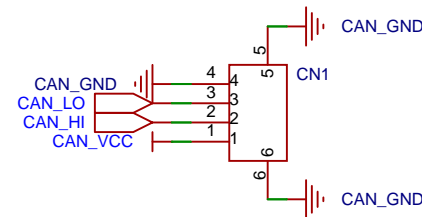
BM04B-GHS-TBT(LF)(SN)
