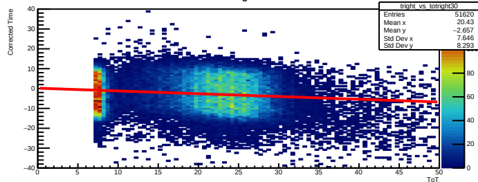
Time Walk right bar=30
