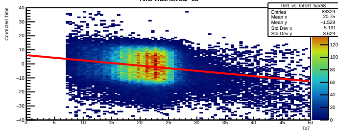
Time Walk left bar=58
