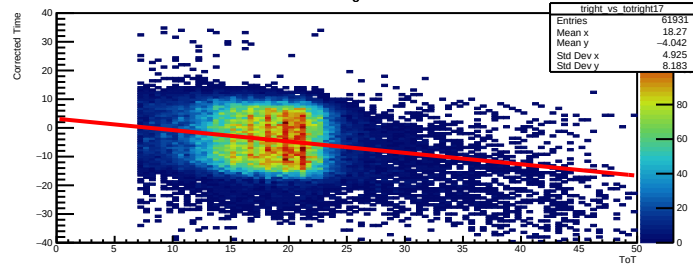
Time Walk right bar=17
