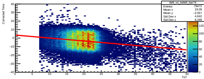
Time Walk left bar=74
