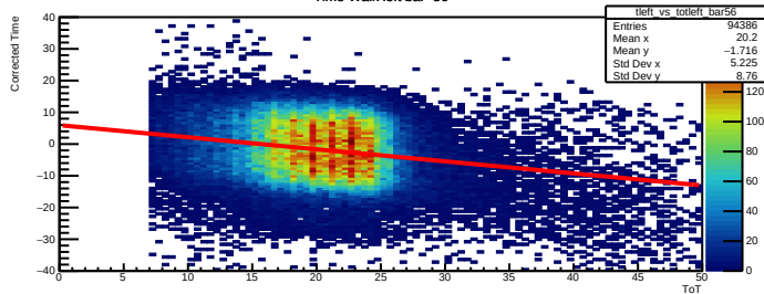
Time Walk left bar=56
