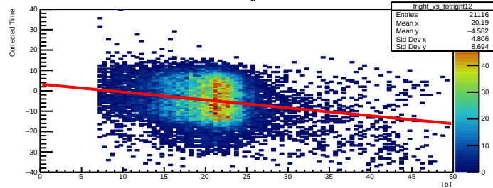
Time Walk right bar=12
