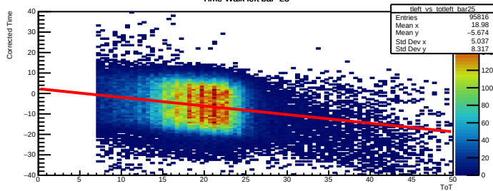
Time Walk left bar=25
