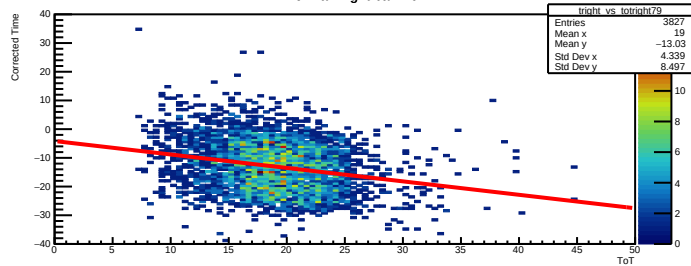
Time Walk right bar=79
