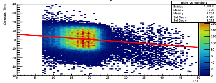
Time Walk right bar=41
