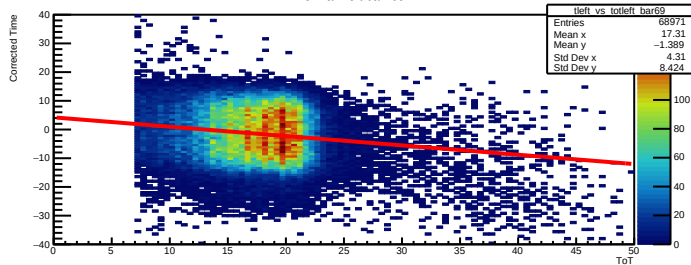
Time Walk left bar=69
