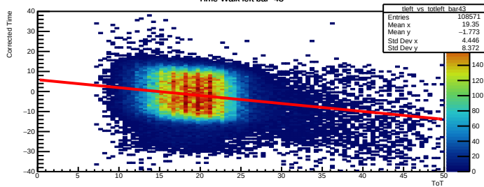
Time Walk left bar=43
