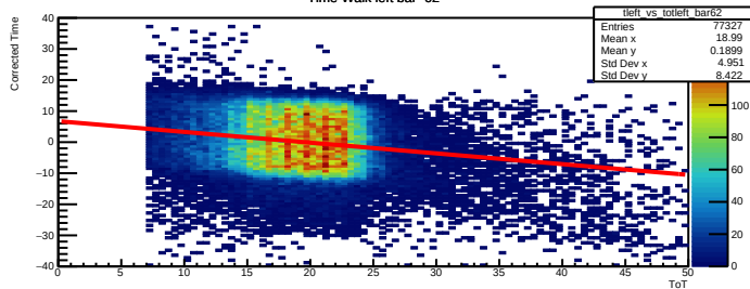
Time Walk left bar=62
