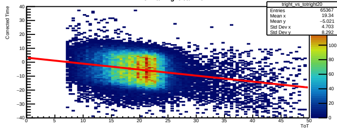
Time Walk right bar=20
