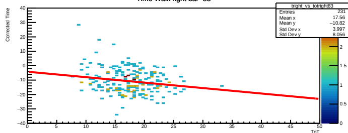
Time Walk right bar=83
