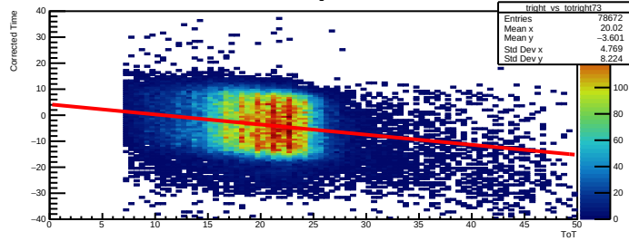
Time Walk right bar=73
