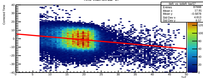
Time Walk left bar=57
