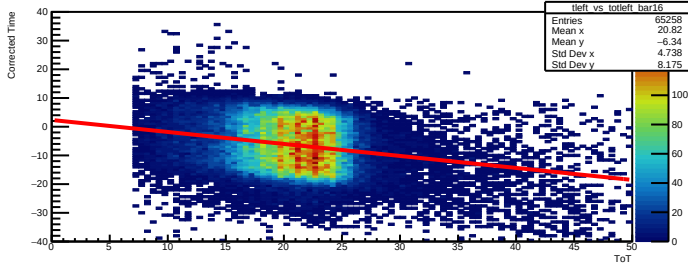
Time Walk left bar=16
