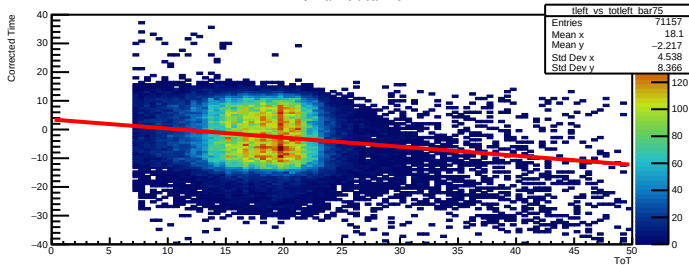
Time Walk left bar=75
