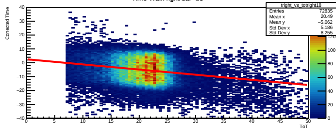
Time Walk right bar=18
