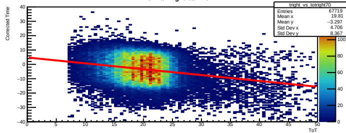
Time Walk right bar=70
