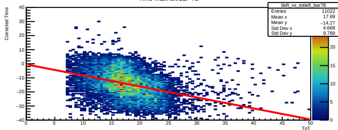
Time Walk left bar=78
