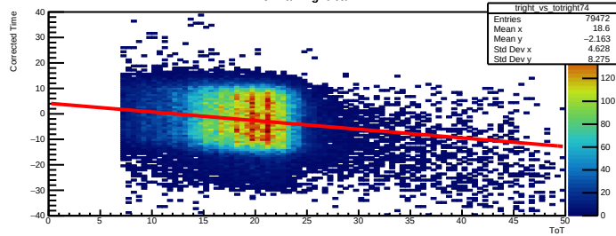
Time Walk right bar=74
