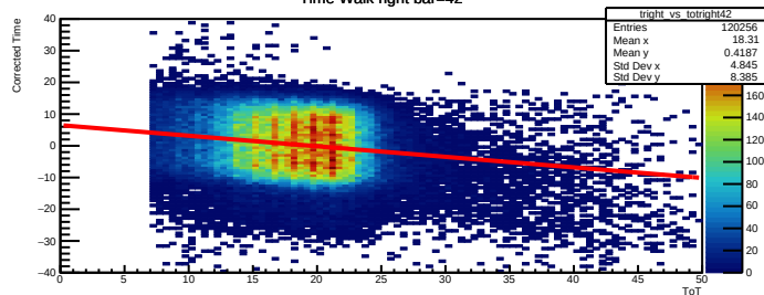
Time Walk right bar=42
