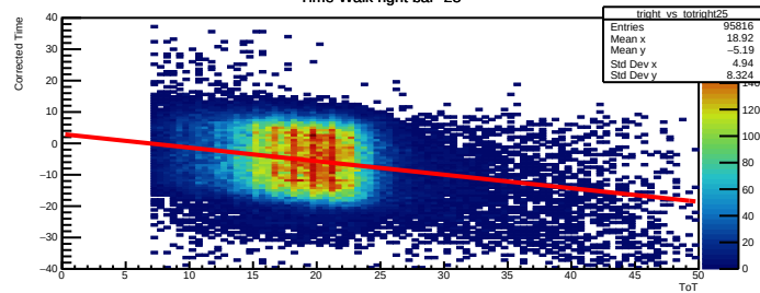
Time Walk right bar=25
