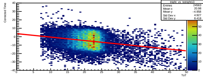
Time Walk right bar=13
