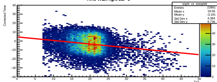
Time Walk right bar=9
