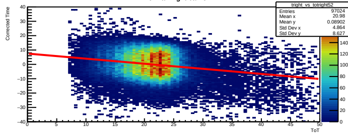
Time Walk right bar=52
