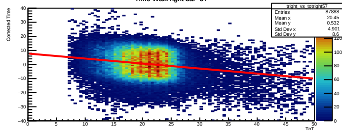
Time Walk right bar=57
