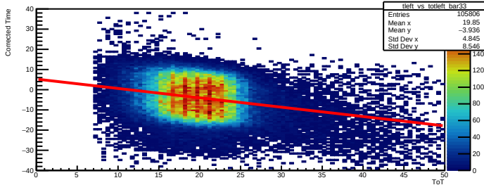
Time Walk left bar=33
