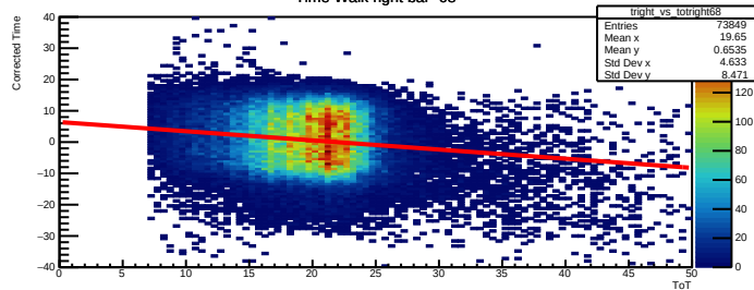
Time Walk right bar=68
