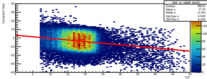
Time Walk left bar=31
