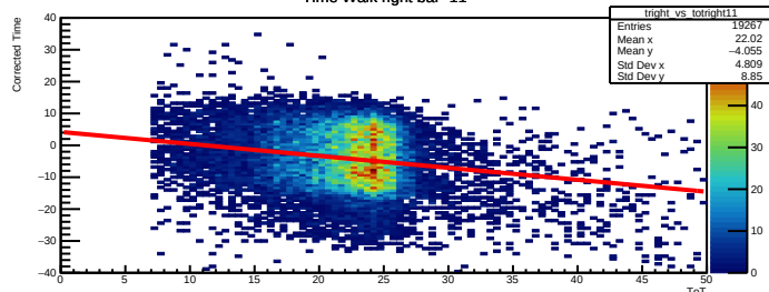
Time Walk right bar=11
