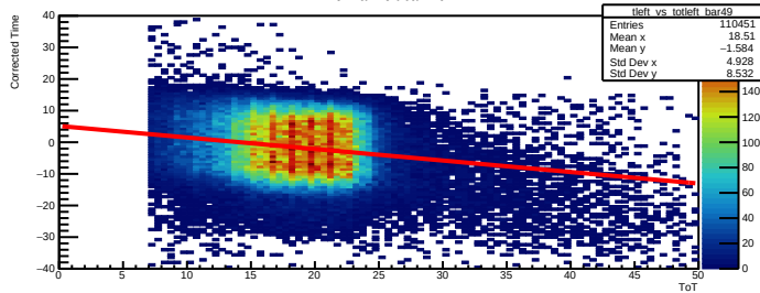
Time Walk left bar=49
