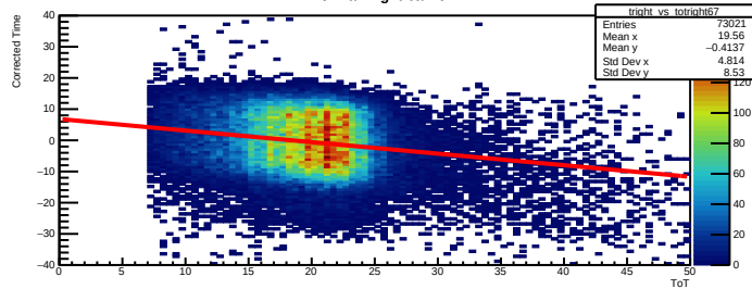
Time Walk right bar=67
