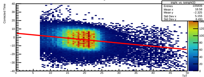
Time Walk right bar=33
