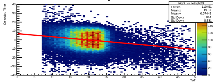
Time Walk right bar=49
