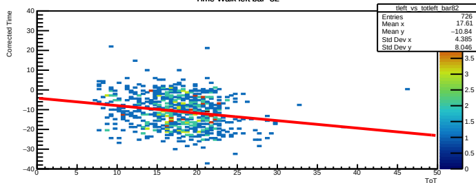
Time Walk left bar=82
