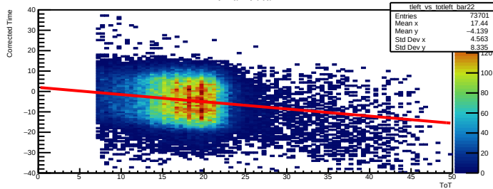
Time Walk left bar=22
