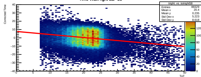
Time Walk right bar=58
