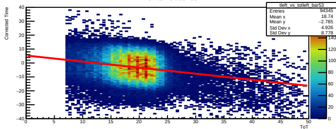
Time Walk left bar=53
