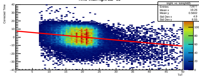
Time Walk right bar=65
