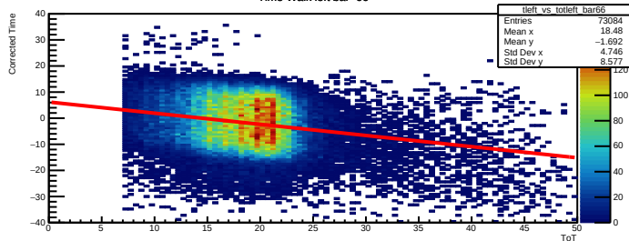
Time Walk left bar=66
