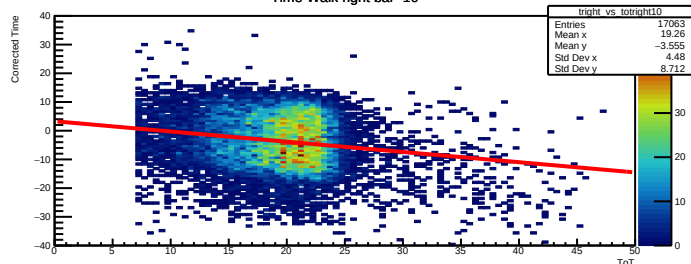
Time Walk right bar=10
