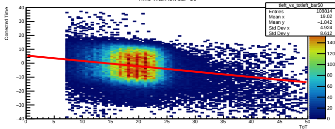
Time Walk left bar=50
