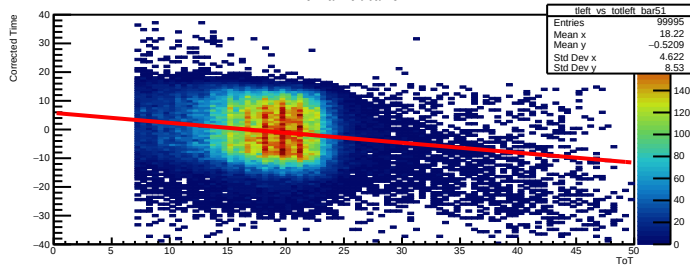
Time Walk left bar=51
