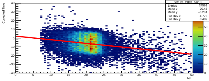
Time Walk left bar=13
