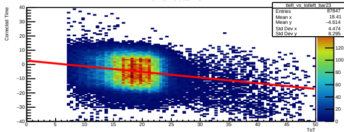
Time Walk left bar=23
