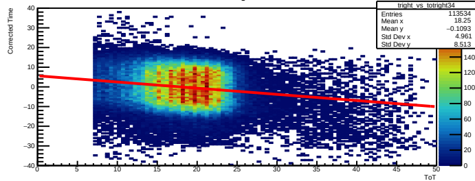
Time Walk right bar=34
