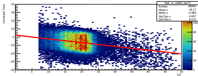
Time Walk left bar=71
