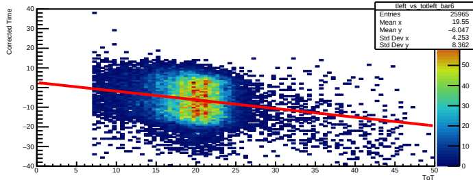
Time Walk left bar=6
