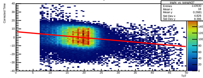
Time Walk right bar=37
