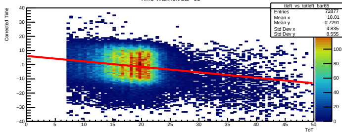
Time Walk left bar=65
