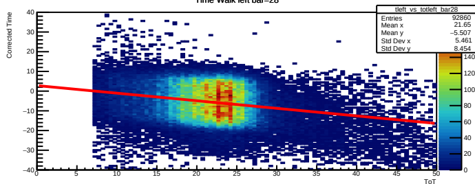
Time Walk left bar=28
