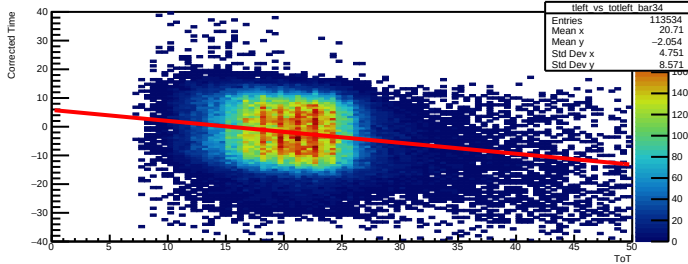
Time Walk left bar=34
