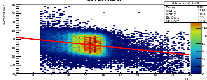
Time Walk left bar=26
