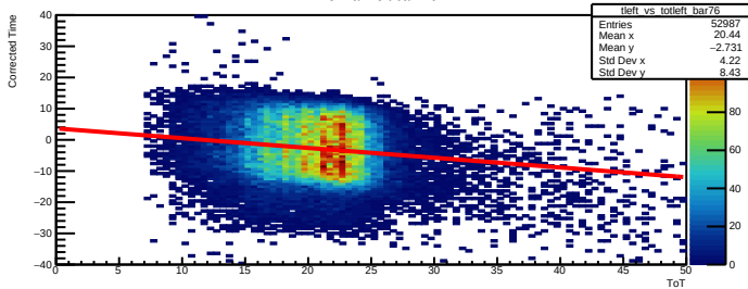
Time Walk left bar=76
