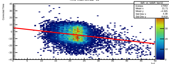
Time Walk left bar=10
