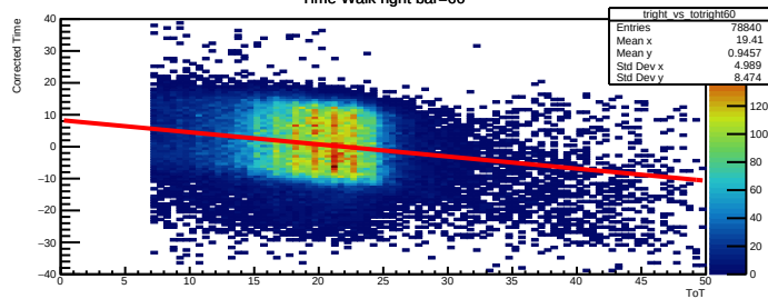
Time Walk right bar=60
