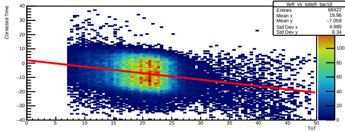
Time Walk left bar=19
