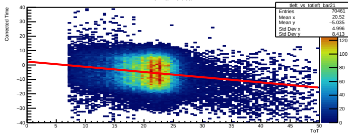
Time Walk left bar=21
