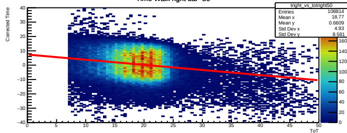
Time Walk right bar=50
