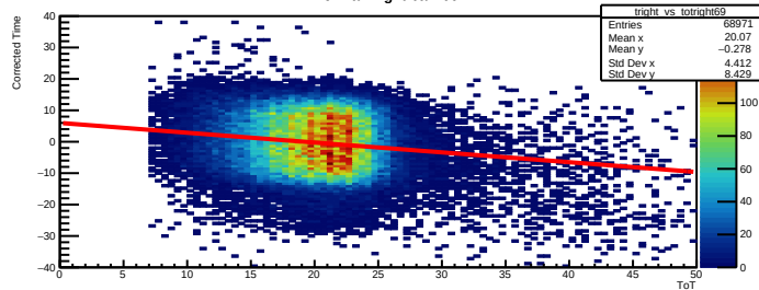
Time Walk right bar=69
