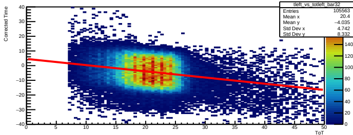
Time Walk left bar=32
