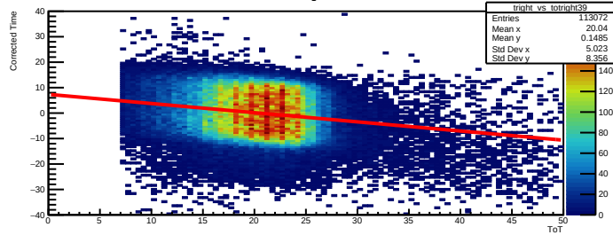
Time Walk right bar=39
