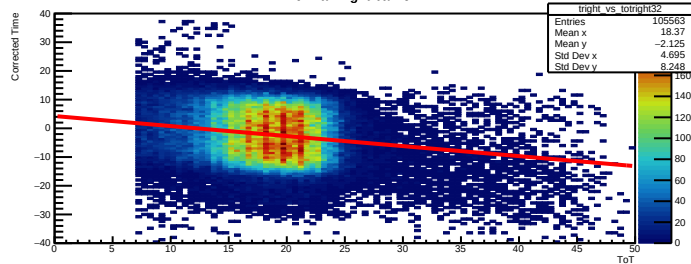
Time Walk right bar=32
