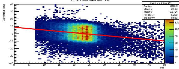
Time Walk right bar=61
