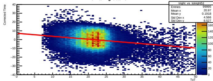
Time Walk right bar=51
