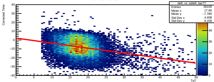
Time Walk left bar=77
