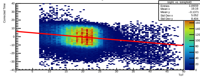
Time Walk right bar=40
