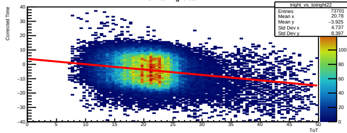
Time Walk right bar=22
