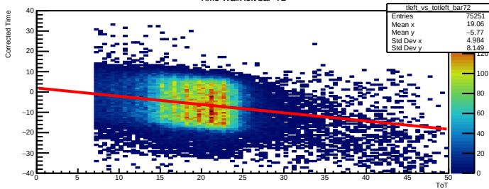
Time Walk left bar=72
