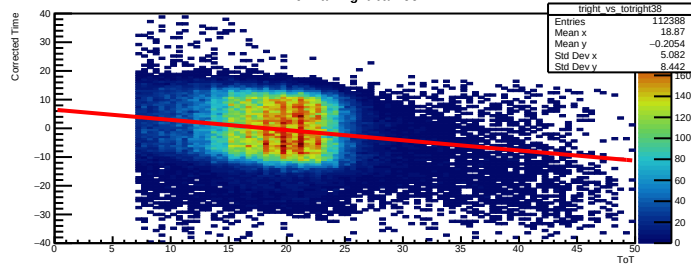
Time Walk right bar=38
