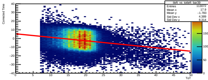
Time Walk left bar=39
