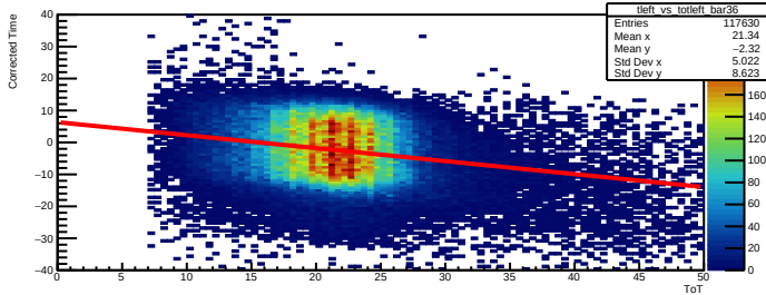
Time Walk left bar=36
