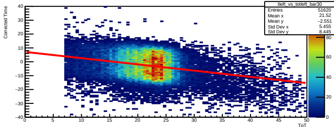
Time Walk left bar=30
