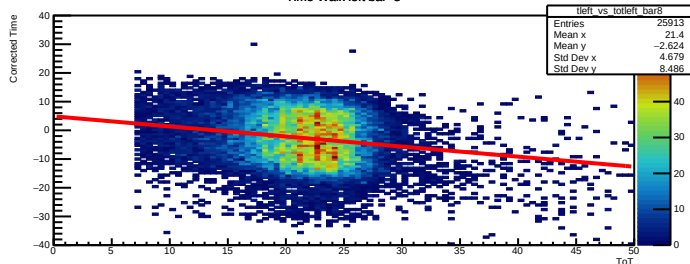
Time Walk left bar=8
