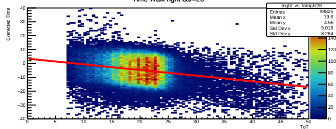
Time Walk right bar=26
