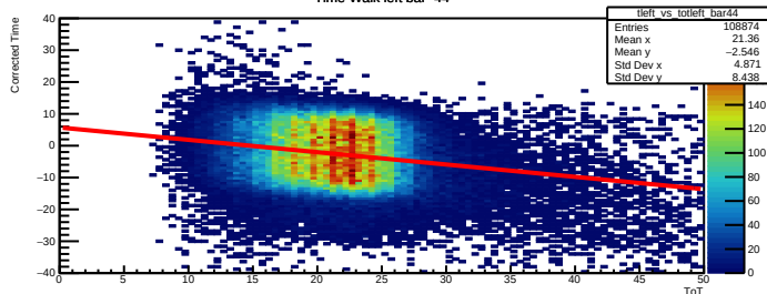
Time Walk left bar=44
