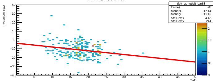
Time Walk left bar=83
