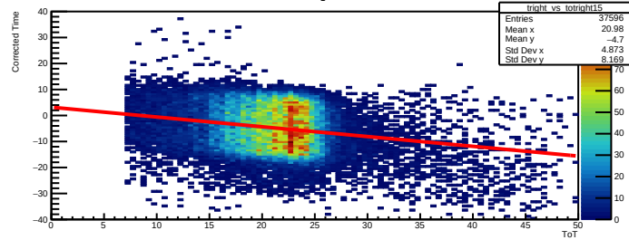
Time Walk right bar=15
