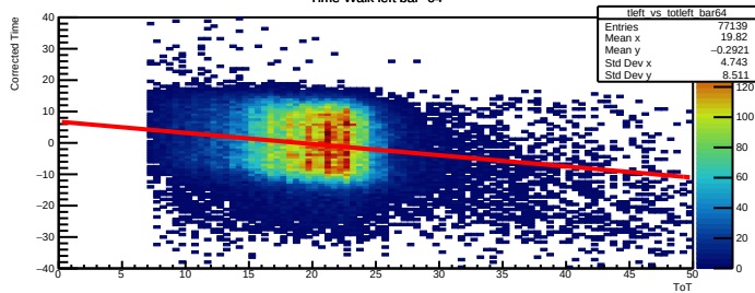
Time Walk left bar=64
