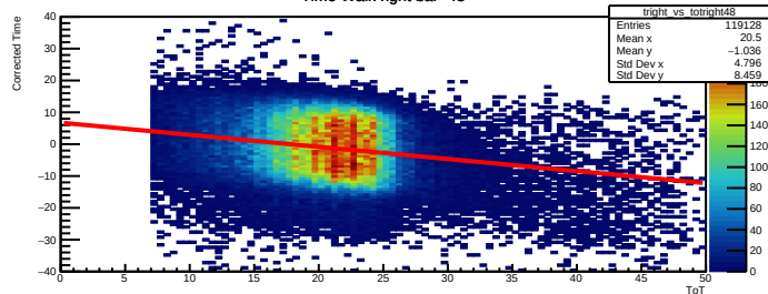
Time Walk right bar=48
