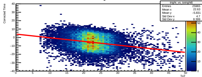
Time Walk right bar=6
