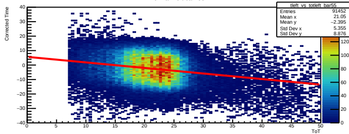
Time Walk left bar=55
