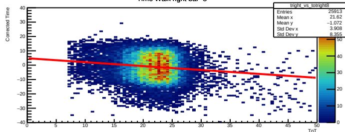
Time Walk right bar=8
