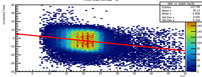
Time Walk left bar=45
