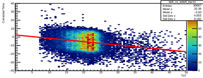
Time Walk left bar=14
