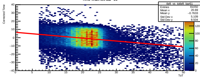
Time Walk left bar=61
