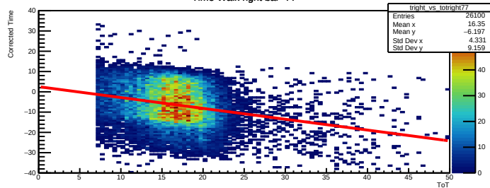
Time Walk right bar=77
