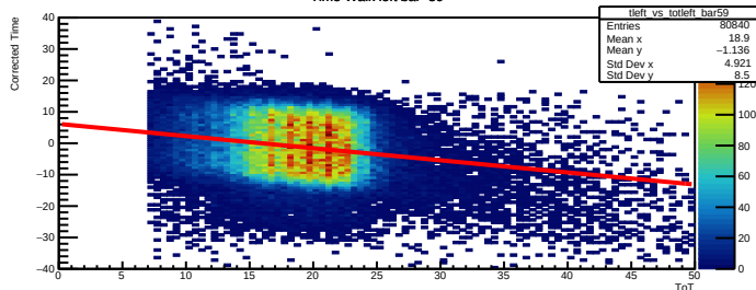
Time Walk left bar=59
