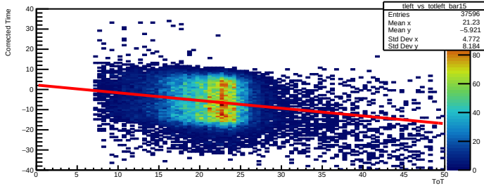
Time Walk left bar=15
