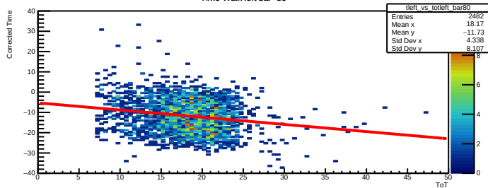
Time Walk left bar=80
