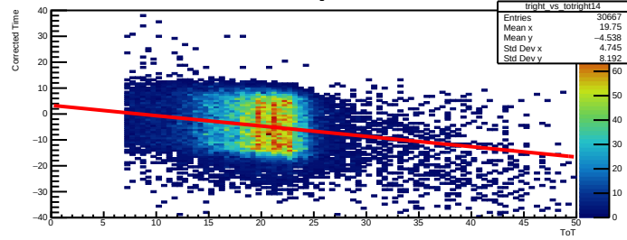
Time Walk right bar=14
