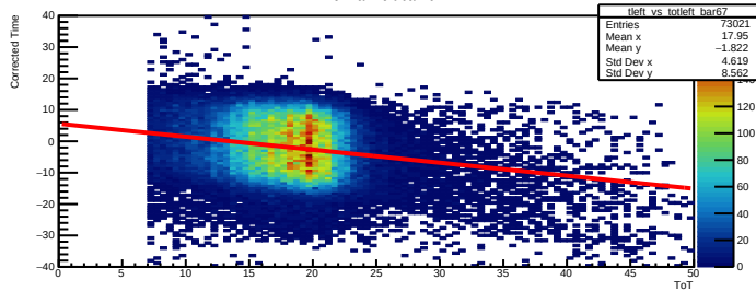
Time Walk left bar=67
