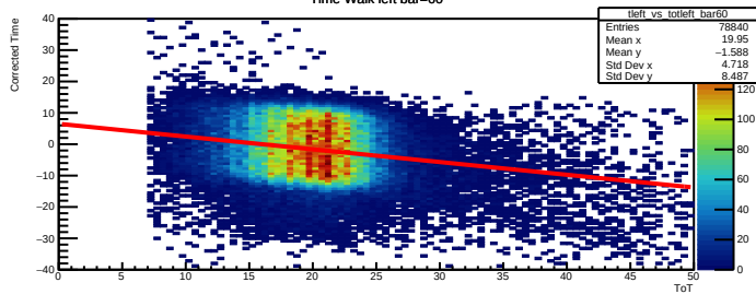
Time Walk left bar=60
