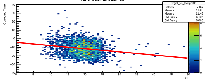
Time Walk right bar=80
