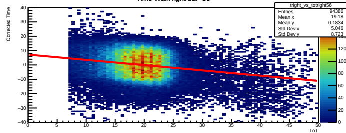
Time Walk right bar=56
