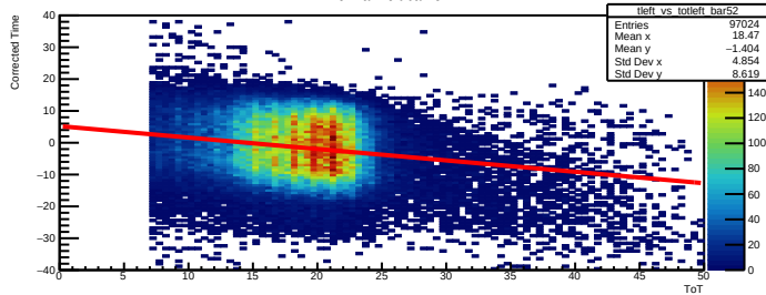
Time Walk left bar=52
