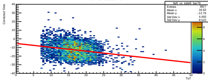
Time Walk left bar=79
