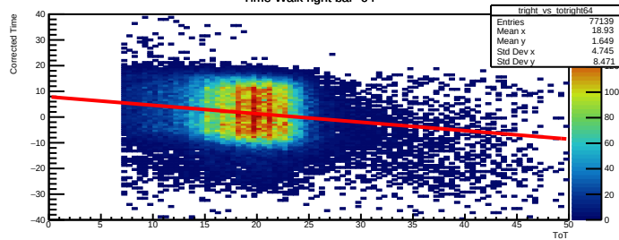
Time Walk right bar=64
