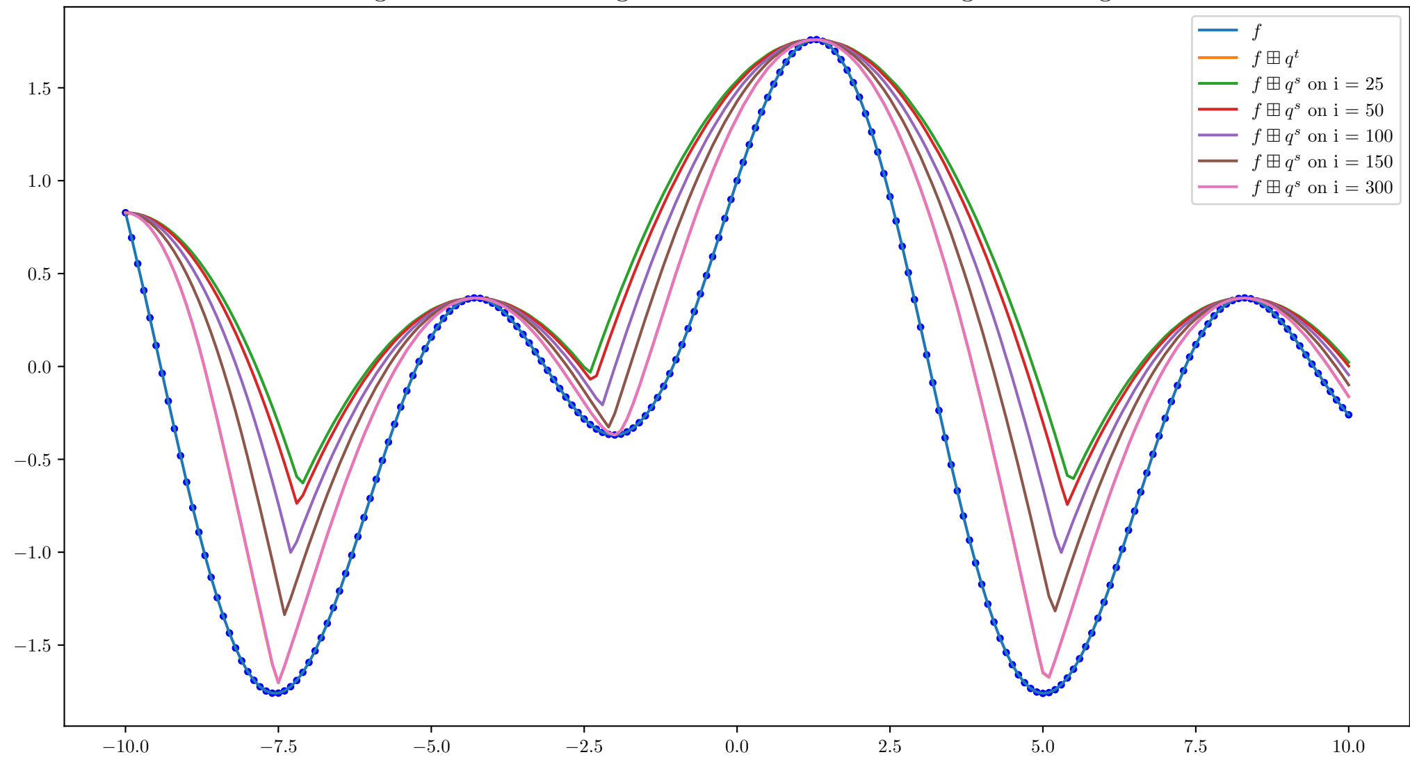
Learning the scale of dilating with t = 50 and the starting scale being 150.0.
