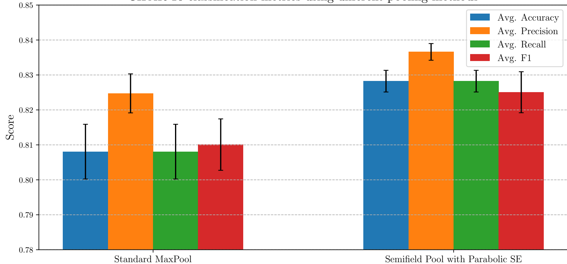
CIFAR-10 classification metrics using different pooling methods
