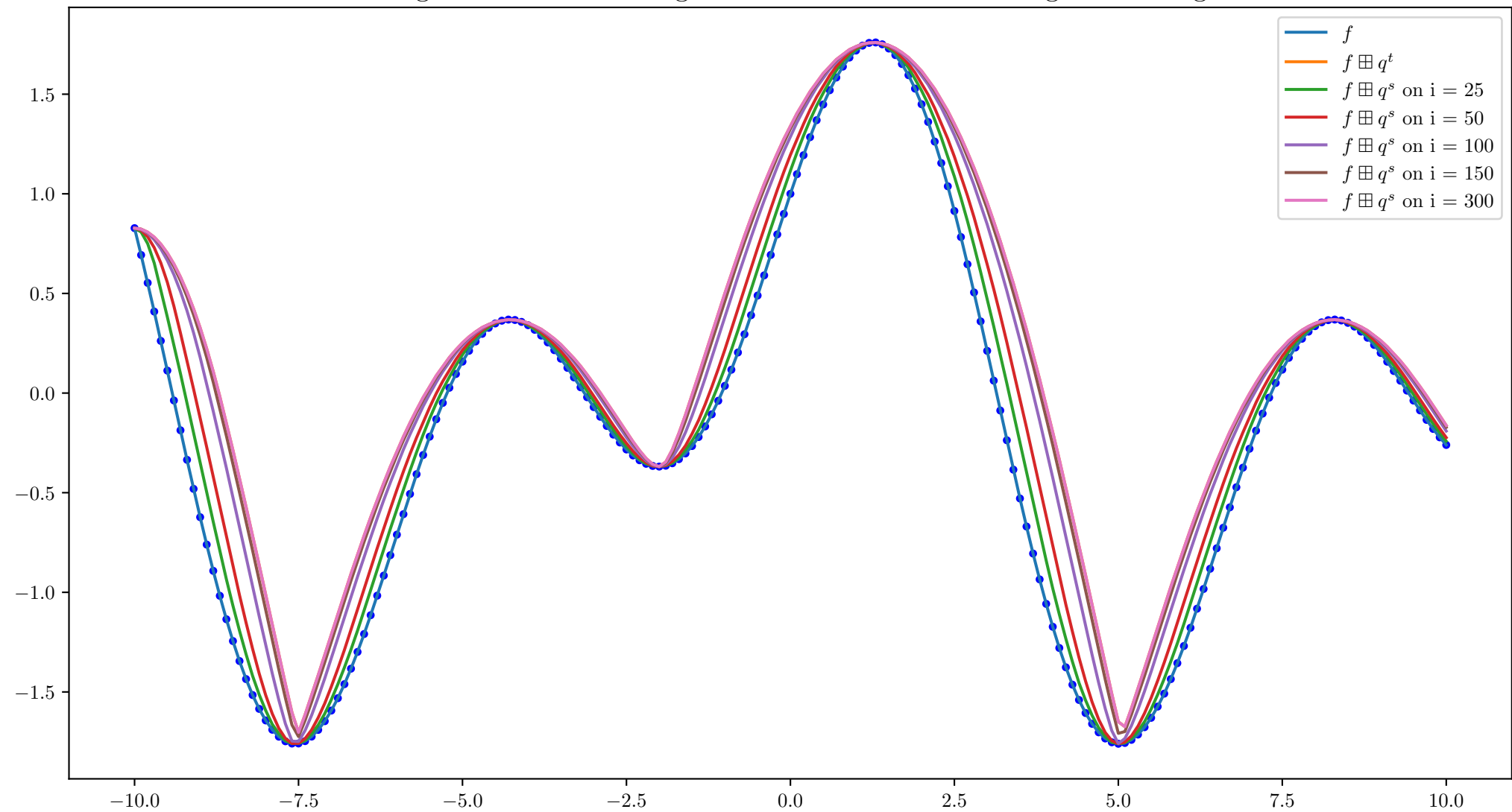
Learning the scale of dilating with t = 50 and the starting scale being 2.0.
