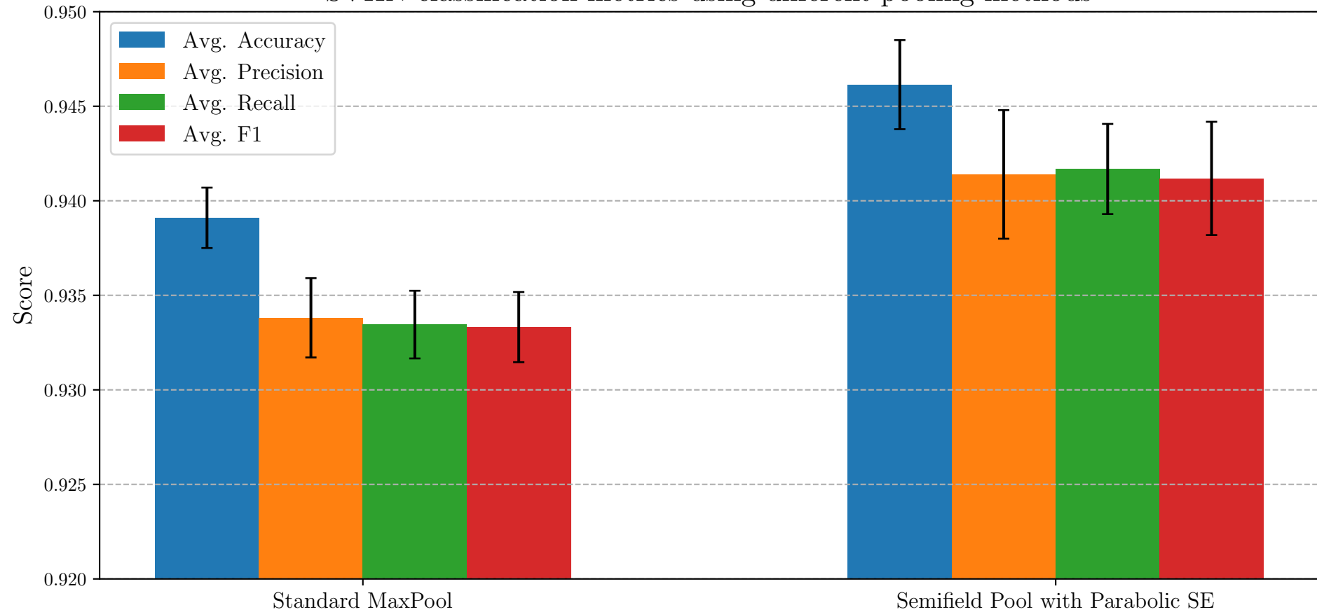
SVHN classification metrics using different pooling methods
