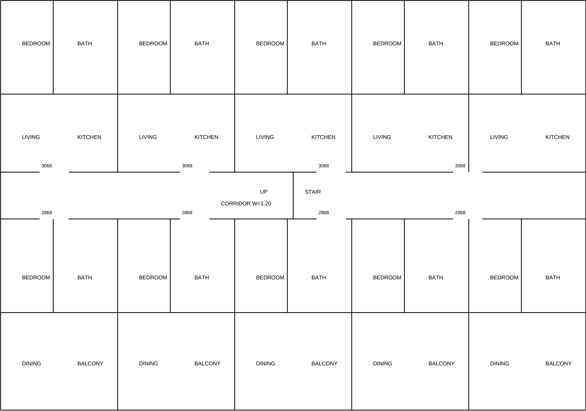
A-101 FIRST FLOOR PLAN
