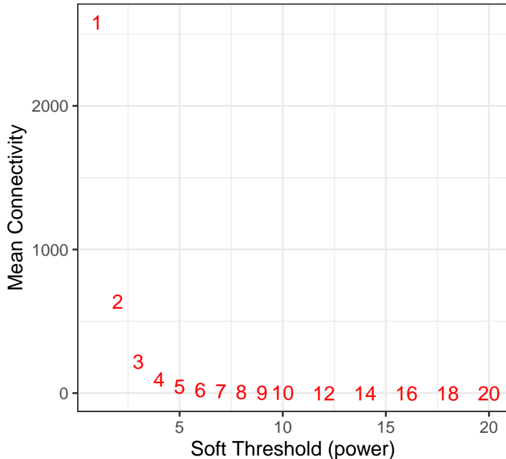
Mean Connectivity
