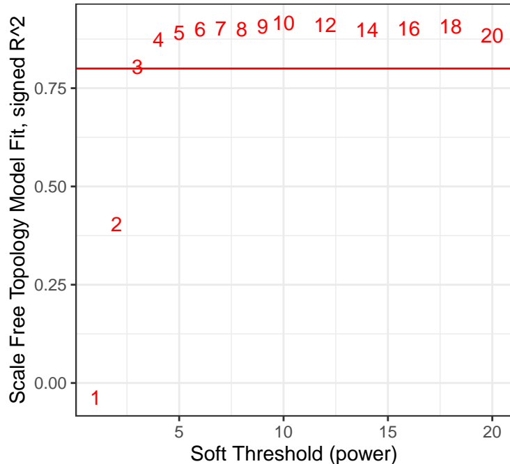
Scale independence
