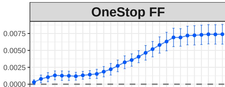
Delta Log Likelihood (average per word)
