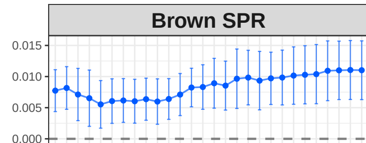
Delta Log Likelihood (average per word)
