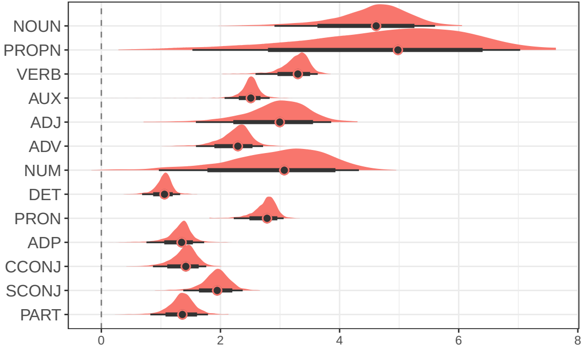
Reduction in Surprisal by Extending Context
