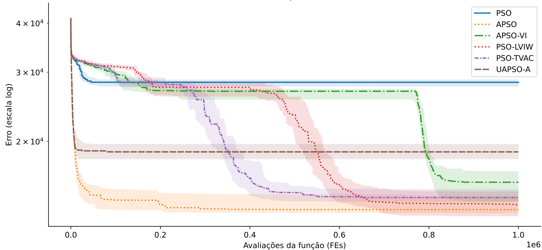
F9 — Levy, Dim: 100
