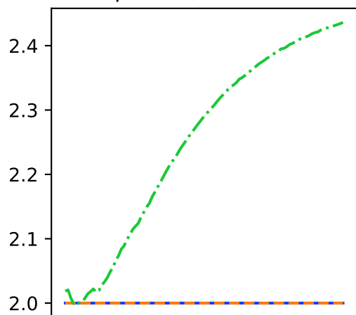
Sphere (dim = 30)
