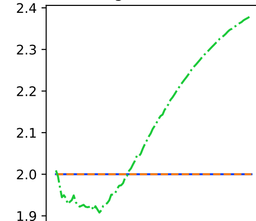
Rastrigin (dim = 100)
