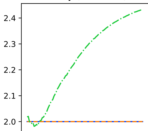
Ackley (dim = 30)
