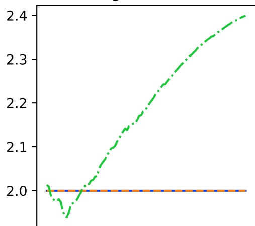
Rastrigin (dim = 30)
