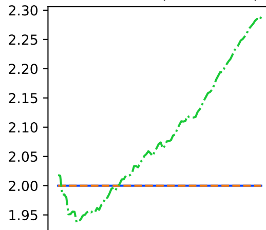
Rosenbrock (dim = 100)
