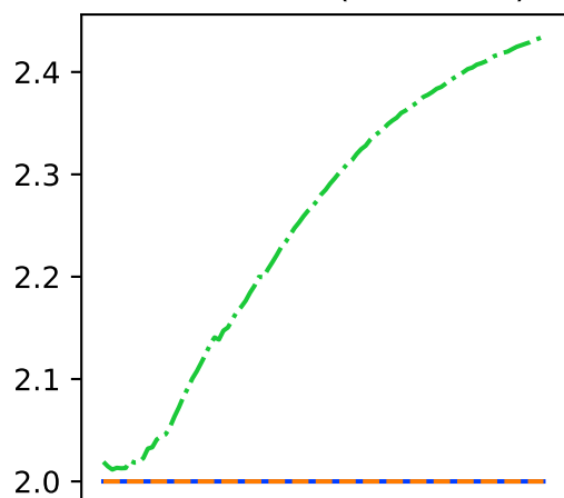
Rosenbrock (dim = 30)
