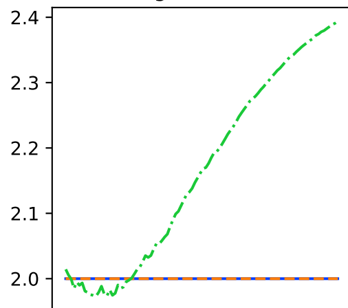
Rastrigin (dim = 50)
