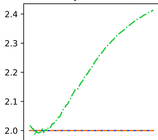
Ackley (dim = 50)
