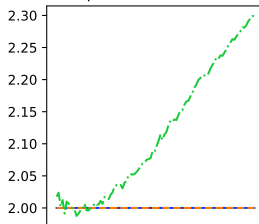
Sphere (dim = 100)
