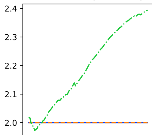
Rosenbrock (dim = 50)
