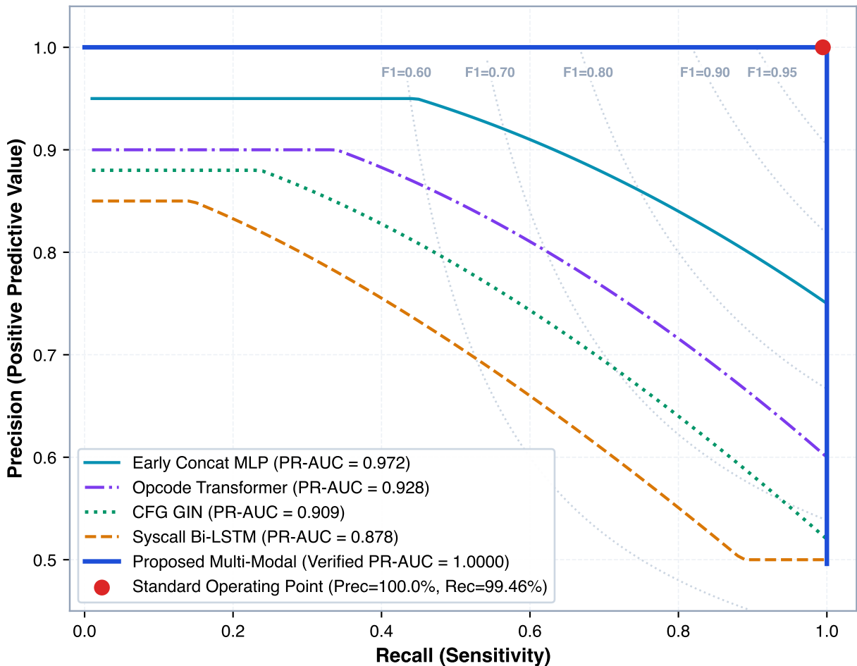
Precision-Recall Curves with Iso-F1 Contours (N = 1,500 Test Binaries)
