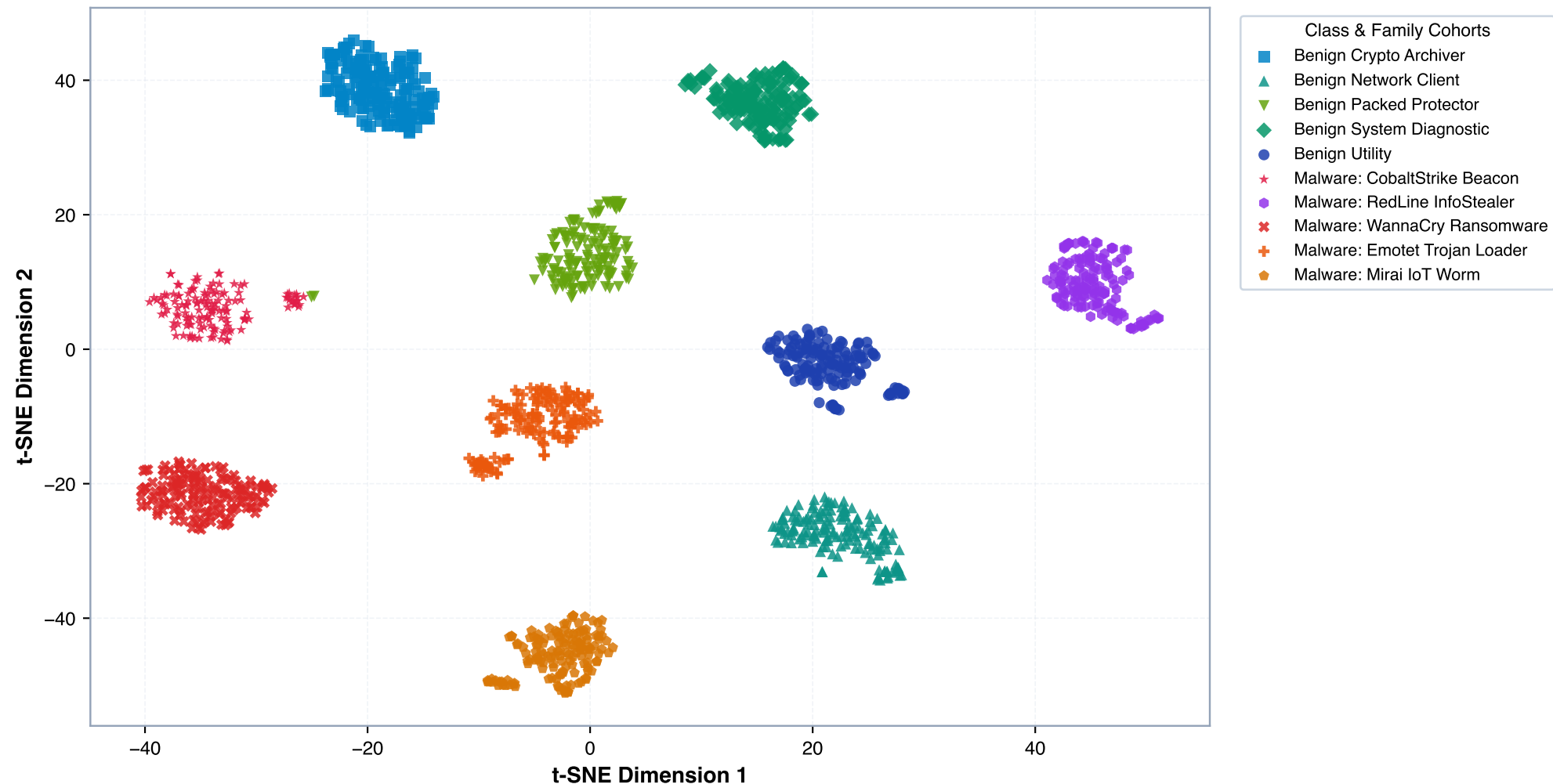
2D Latent Representation Manifold (t-SNE, Perplexity = 30, N = 1,500 Test Samples)
