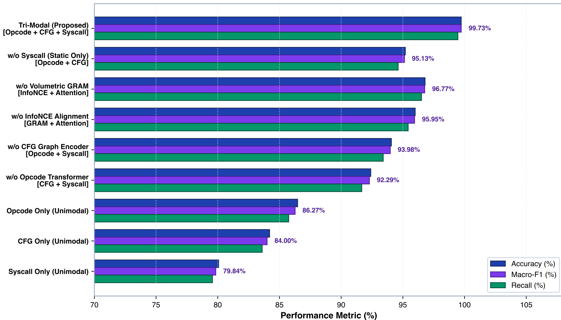
Modality and Alignment Ablation Evaluation (Held-Out Test Set, N = 1,500)
