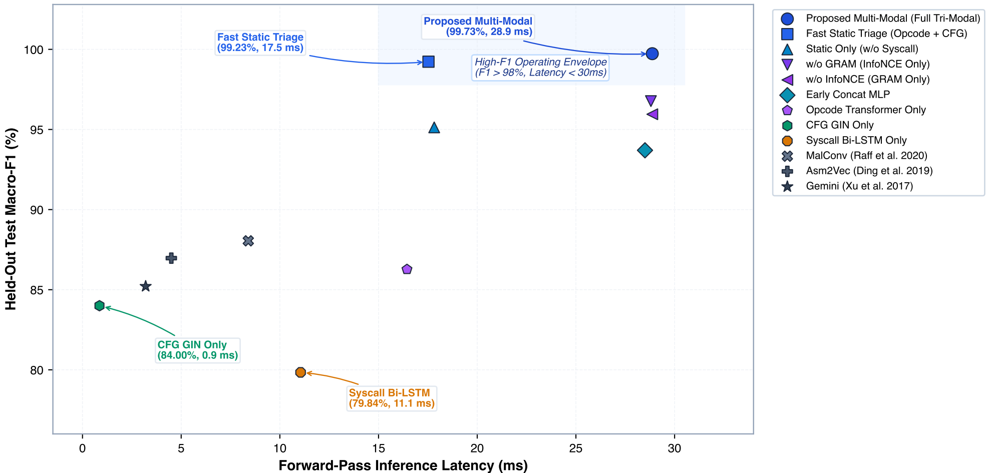
Inference Latency vs. Classification Macro-F1 Trade-Off Across Evaluated Architectures
