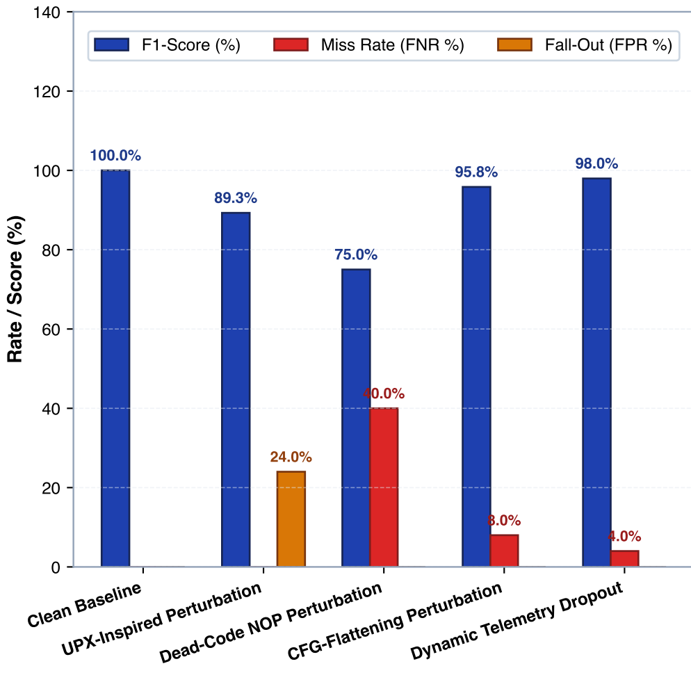
(a) Detection Robustness under Simulated Perturbations (N=1,000)
