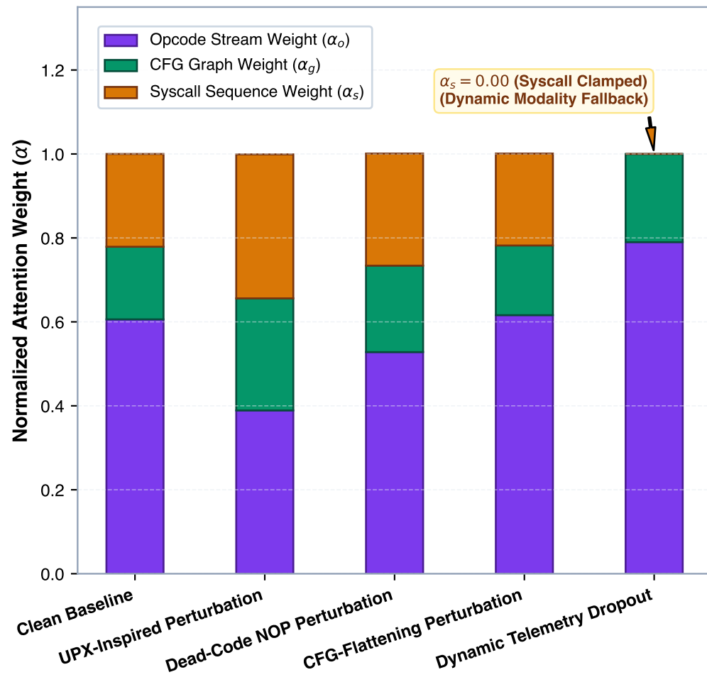
(b) Dynamic Attention Weight Reallocation
