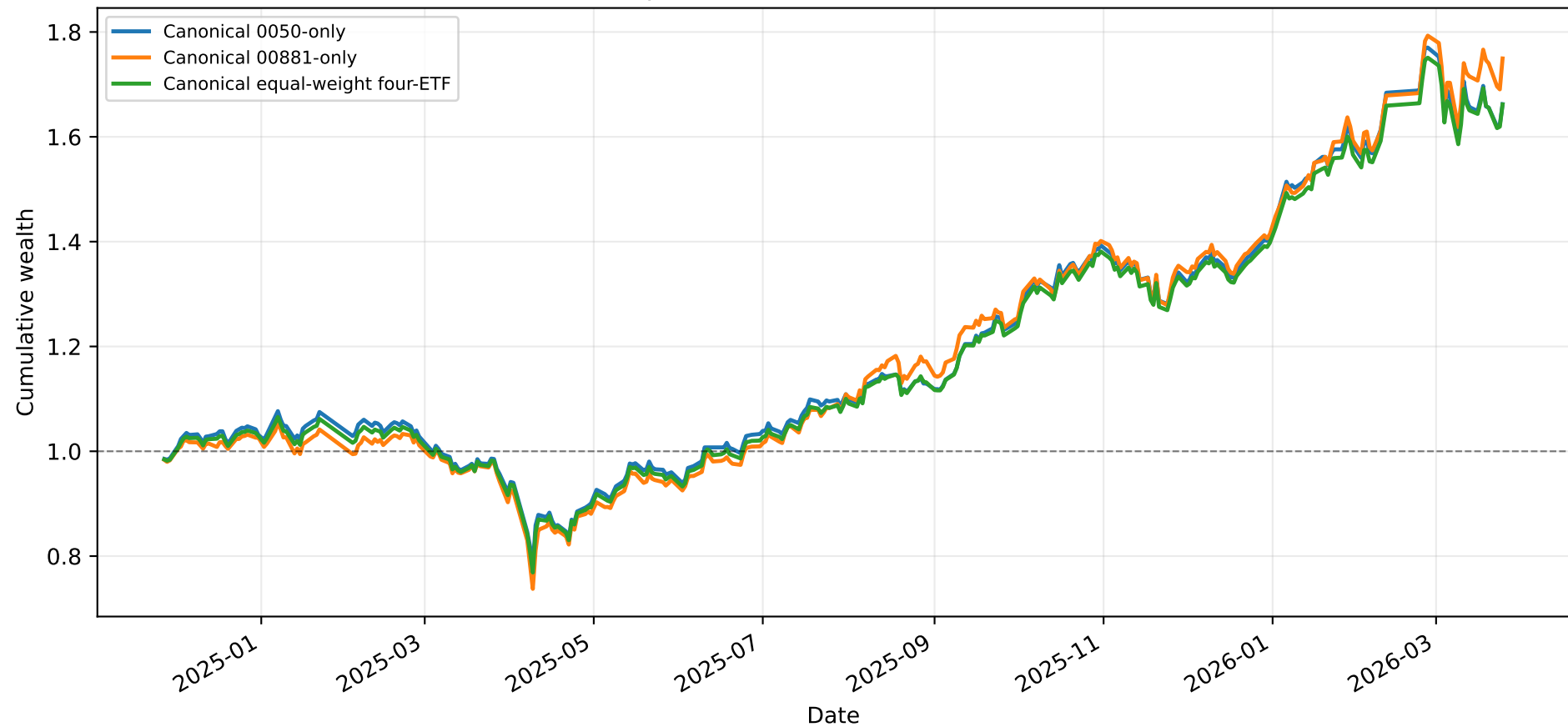
Canonical passive benchmark cumulative wealth
