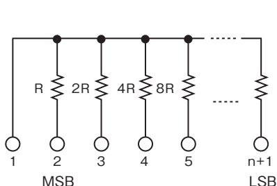
K circuit
