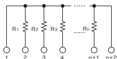
D circuit
