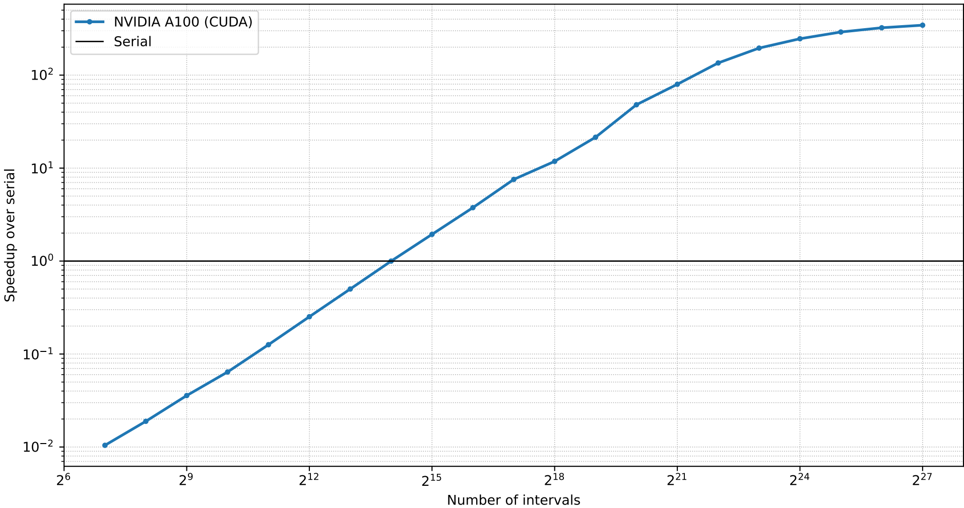
Kokkos speedup over serial: scalar integration
