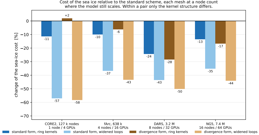
Figure 1: Cost of the sea ice relative to the standard scheme; negative is a saving. Each mesh is at its operating point, the largest node count at which the model still gains from more GPUs. Within each pair of bars the ring, the messages and the bytes are identical — only the kernel structure differs.
