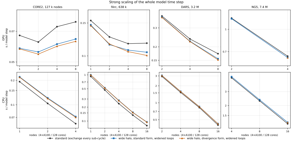
Figure 2: Strong scaling of the whole model time step. Lower is better.
