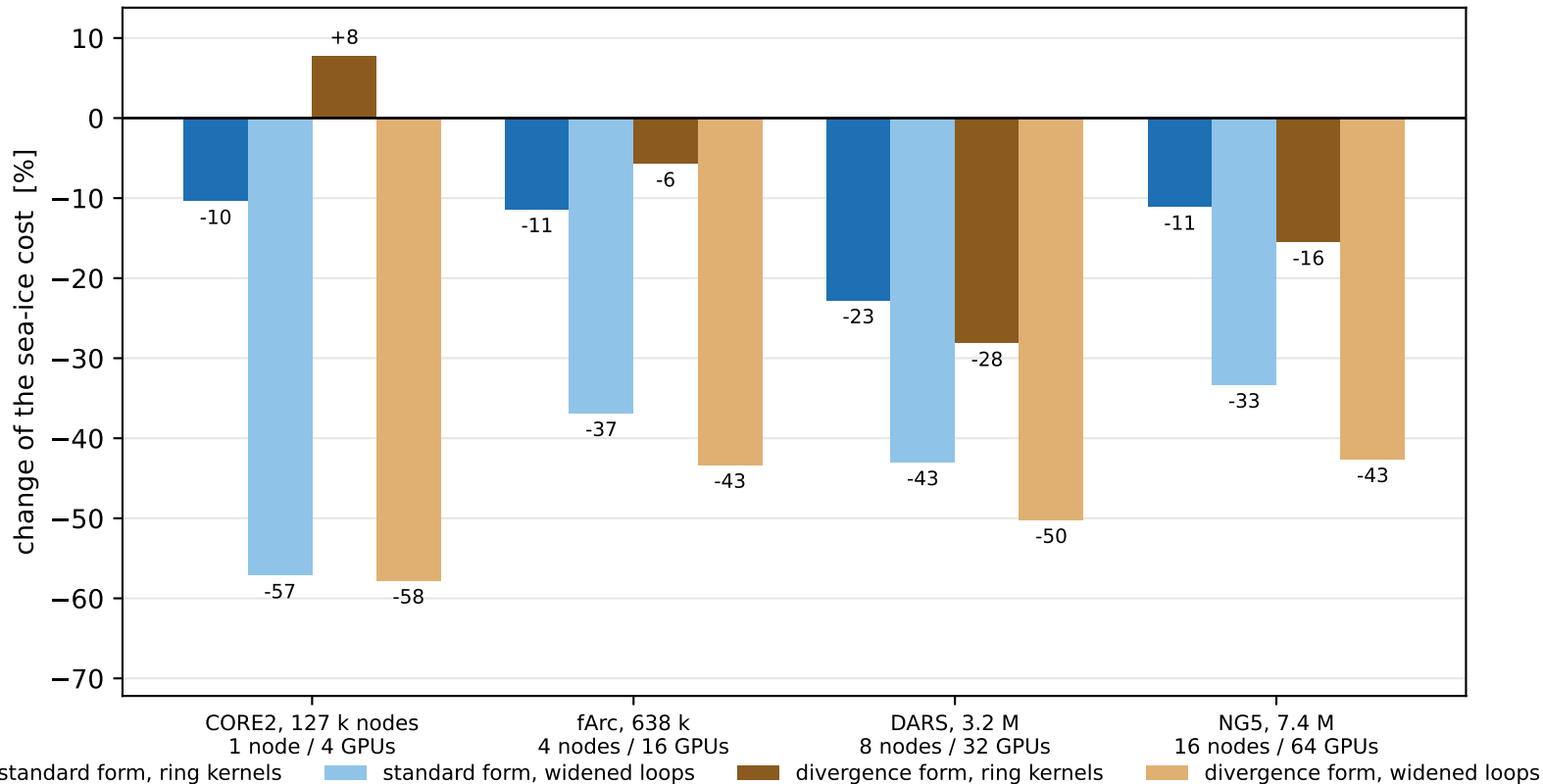
Cost of the sea ice relative to the standard scheme, each mesh at a node count where the model still scales. Within a pair only the kernel structure differs.
