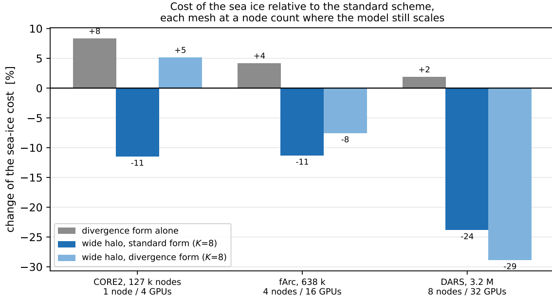
Figure 1: Cost of the sea ice relative to the standard scheme, for the schemes that survive Sect. 6.6. Negative is a saving. The measure is the ice cost — ice, ice dynamics and ice advection, computation together with time spent waiting for communication — and not the model time step, which divides an ice-only change by about ten. Each mesh is at its own operating point, the largest node count at which the model still gains from more GPUs, read off the measured strong-scaling curve of the standard scheme; each was measured in a single allocation with all configurations run back to back. Both wide-halo bars are exact and reproduce the standard trajectory bit for bit.
