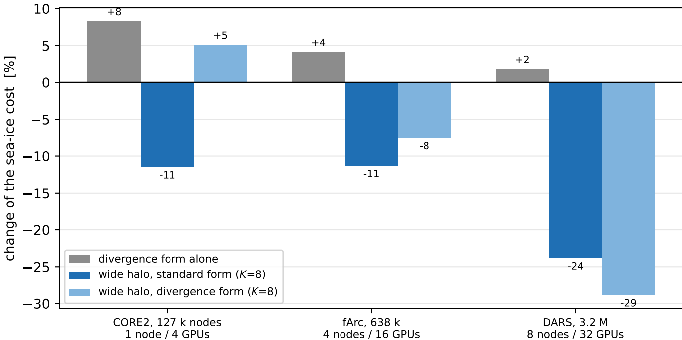
Cost of the sea ice relative to the standard scheme, each mesh at a node count where the model still scales
