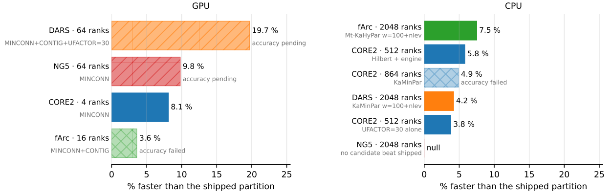
Figure 1: Best candidate partition per mesh and rank count, as a percentage faster than the shipped partition. Gray text under each label is the setting that produced the candidate. Solid bars are certified (stability and accuracy both passed); single-hatched bars await their accuracy test; cross-hatched bars failed it. Mesh colors follow the project’s figure conventions and recur in Figs. 2 and 3.
