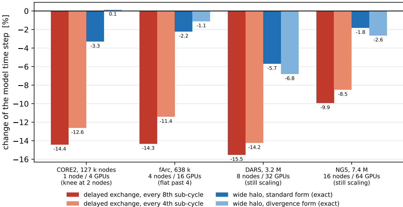
Cost of one model time step relative to the standard scheme, each mesh at a node count where the model still scales
