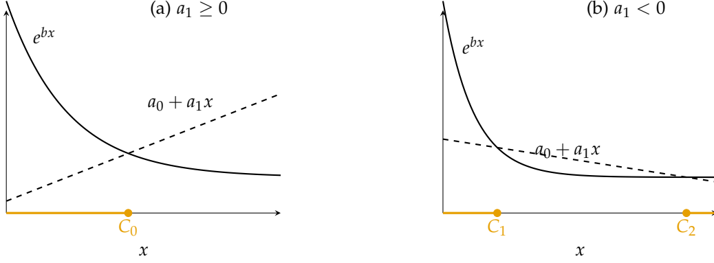
Figure 1: Two possible shapes of the rejection region, highlighted in orange, for the test in eq. (3) when b < 0 , depending on whether a_1 is positive.
