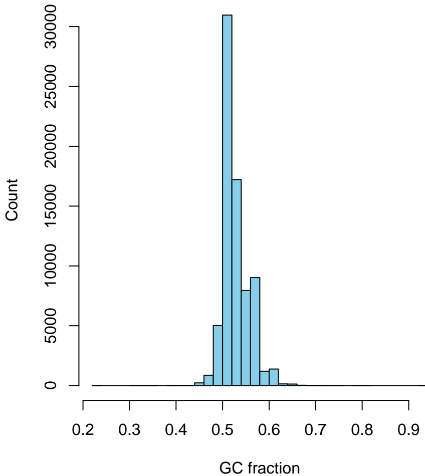
GC Content Distribution
