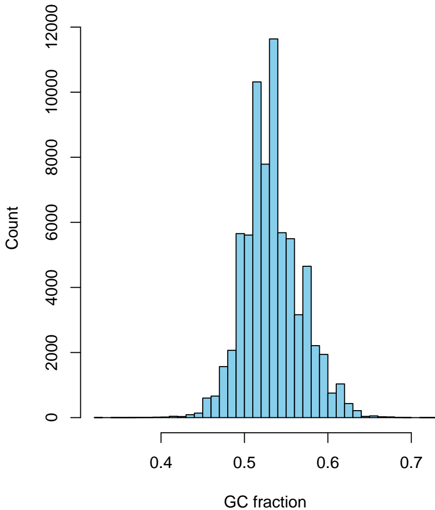
GC Content Distribution
