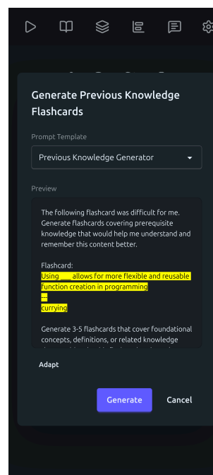
Figure 2: First step of the generation modal. Basic prompt management allows customizing what kind and how many flashcards will be generated.
