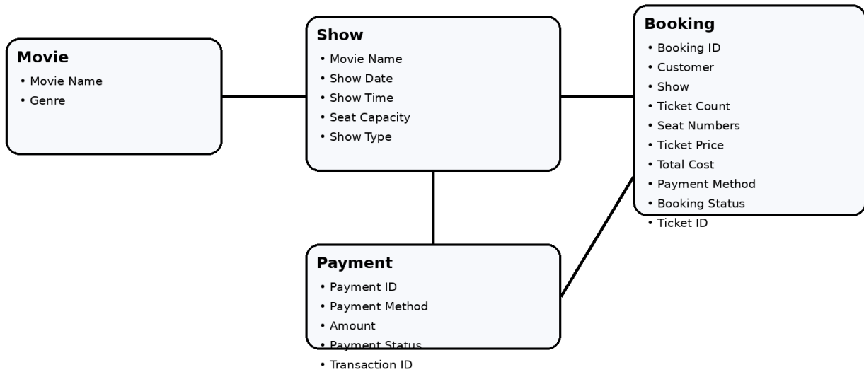
Figure 6. Data object architecture.
