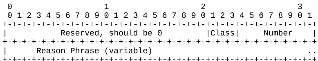
Figure 7: ERROR-CODE Attribute
