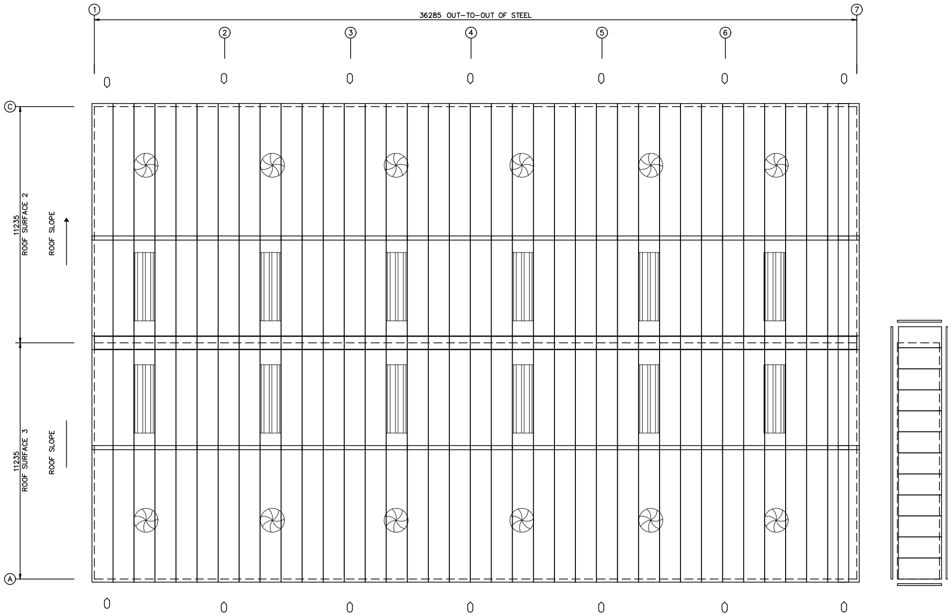
ROOF SHEETING PLAN
